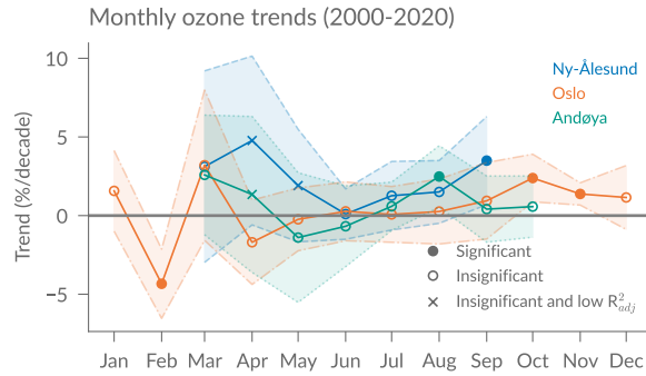
Figure 8. Monthly ozone trends in percent per decade for the three stations, with 2\text{-}\sigma uncertainty shadings. Filled dots represent trends that are significantly different from zero at the 95% confidence interval. Fits with low R_{adj}^2 < 0.5 are marked with crosses.
