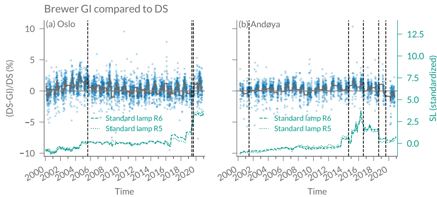
Figure A2. Brewer Global Irradiance (GI) data compared to DS data at (a) Oslo and (b) Andøya. Data smoothed with a moving mean window of 30 days is shown by the thick grey lines. The right axis shows standard lamp (SL) ratios R5 and R6, standardized to zero mean and standard deviation of one, smoothed with a moving mean window of 30 days. Vertical dashed lines show dates that were used for GI calibration.
