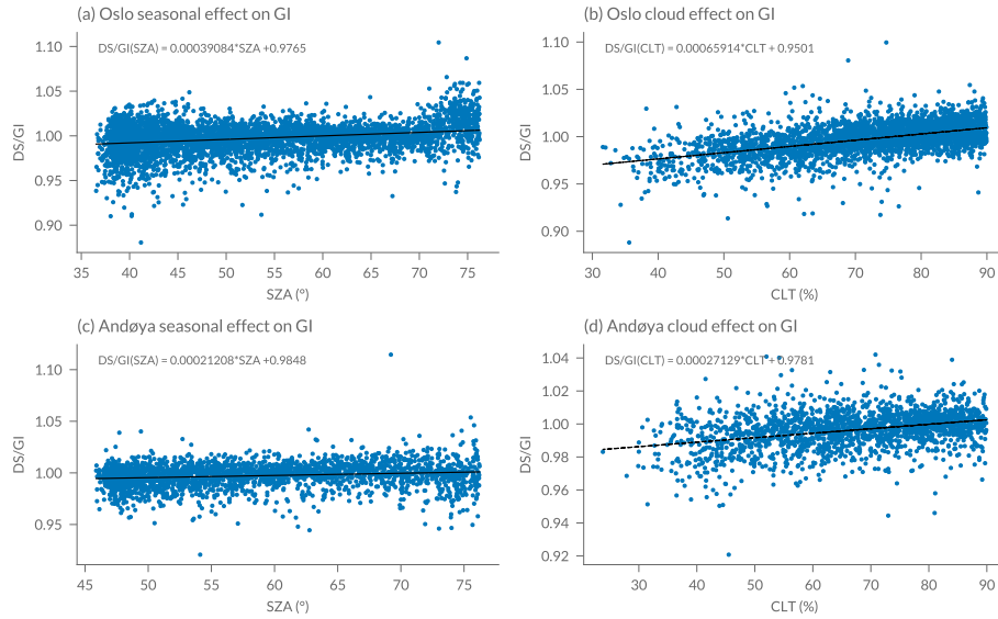
Figure A1. Linear relationships between the DS/GI-ratio and (a,c) the solar angle (SZA) as well as (b,d) the cloud transmittance (CLT) for Oslo (1995 to 2020) and Andøya (2000 to 2020).
