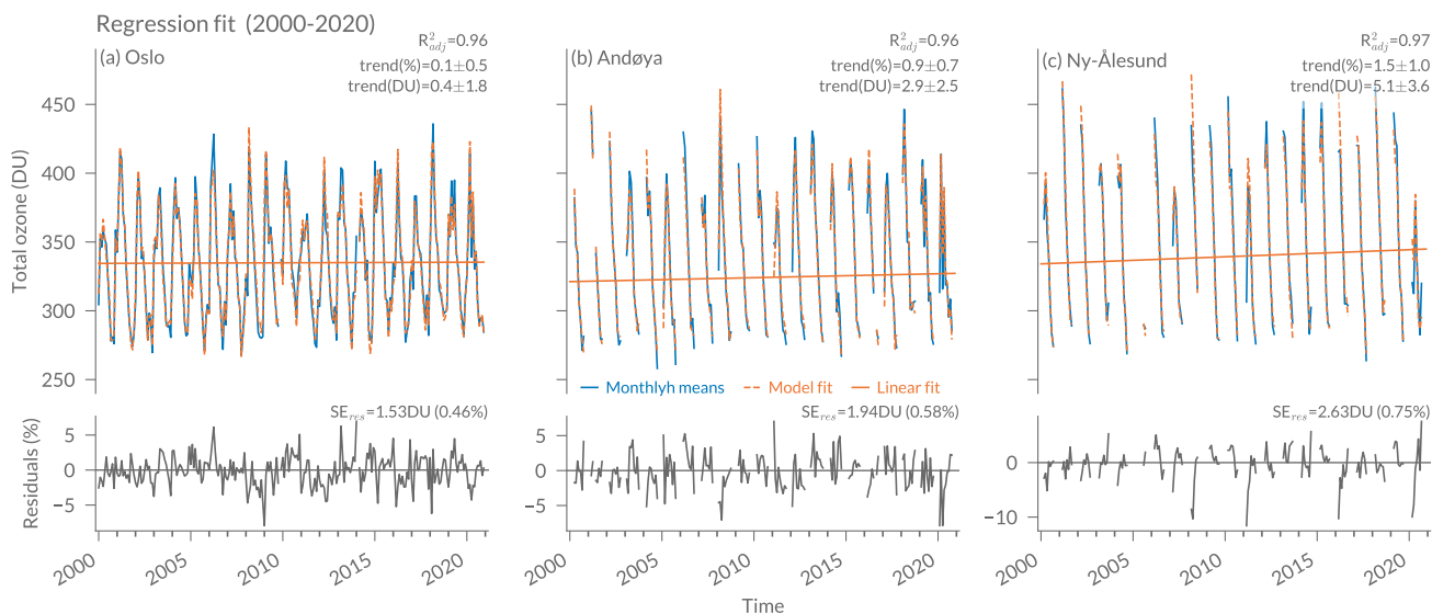
Figure 7. Regression fit of total ozone for (a) Oslo, (b) Andøya, and (c) Ny-Ålesund. The resulting linear trend is given in % per decade and DU per decade with 2-standard-deviation ( \sigma ) uncertainties. The lower panels show the residuals of the regression fit in percent ((Data–Model)/Data) and the standard error of the residuals ( SE_{res} ) in DU and percent (compared to the mean ozone value at each station).
