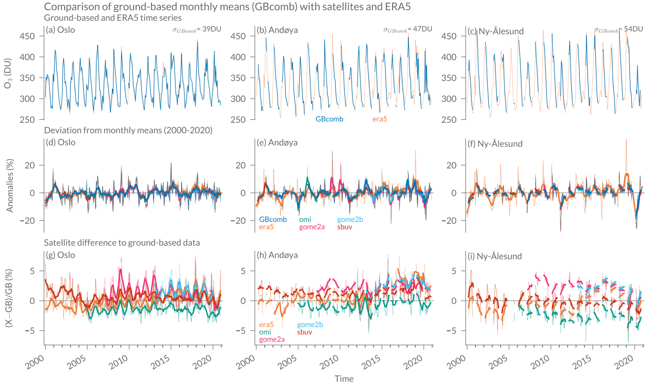
Figure 3. Comparison of the combined ground-based data (GBcomb) with satellite overpasses and ERA5 data at the three stations Oslo, Andøya and Ny-Ålesund. The first row ((a)–(c)) shows monthly means of the ground-based data together with ERA5 monthly means. The standard deviation of GBcomb data ( \sigma_{GBcomb} ) is also given. The second row ((d)–(f)) shows relative anomalies for each dataset, which are defined as the deviation of each month from the monthly mean climatology (2000–2020) of the respective dataset. The third row ((g)–(i)) shows monthly differences between GBcomb and coincident daily means of the other datasets. The thick lines in (d)–(i) show data smoothed with a moving window of 6 months (with a minimum window size of 3 months).
