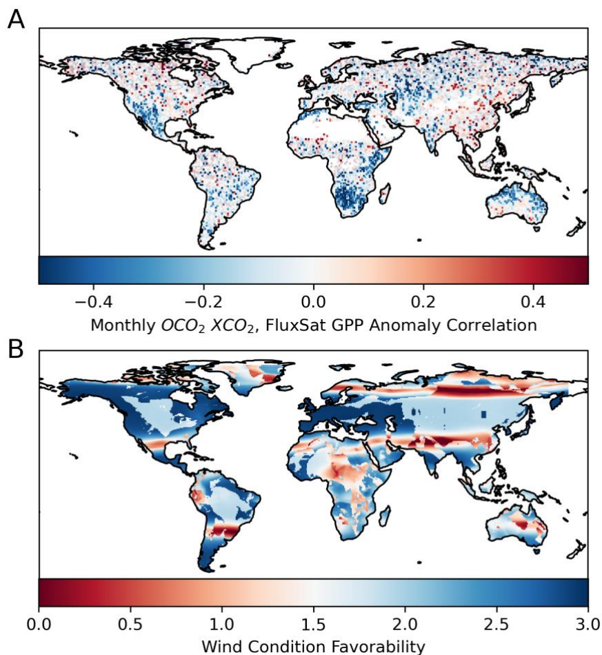
335 Figure 1. (a) Observed coupling between terrestrial biosphere surface CO 2 flux anomalies and atmospheric CO 2 concentration anomalies. Monthly anomaly correlation between observed column CO 2 (XCO 2 ) from OCO-2 and observation-based FluxSat GPP (derived primarily
