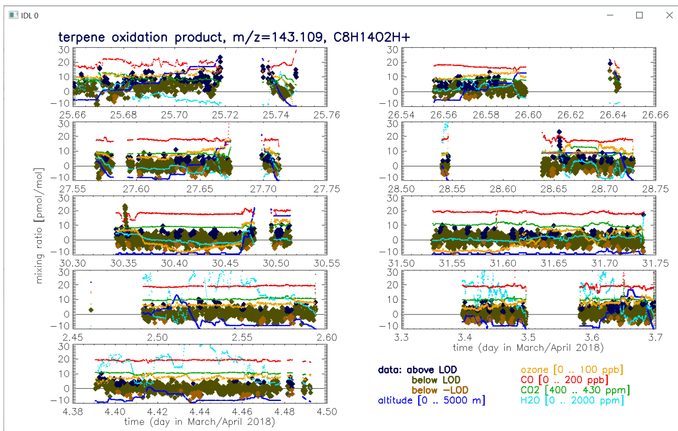
40 Figure S1: Data and presentation as in Figure 3 but for the signal detected at 143.109 Th. The campaign mean (median) mixing ratio was 1.2 (0.7) pmol/mol for this ion. Measured mixing ratios generally did not emerge above the LOD. The measurements plotted in black ( n=812 ) were above the LOD, and values plotted in brown ( n=315 ) were negative below -LOD. The fraction above LOD was calculated by subtracting the 'brown' points from the 'black' points and dividing the result by the total number of measurements ( n=7771 ). The result is 6.4 % for this ion.
