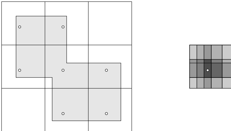
Figure 2: Illustration for the proof of Lemma 1 in \mathbb{R}^2 .
