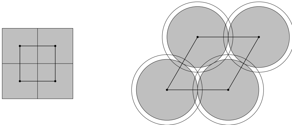
Figure 1: Left: When C is a unit square, a square lattice of cell length 1 supports both a lattice covering by C and a lattice packing of C . Right: When C is a disk of unit radius, a triangular lattice of cell length \sqrt{3} supports both a lattice covering by C and a lattice packing of (\sqrt{3}/2)C .
