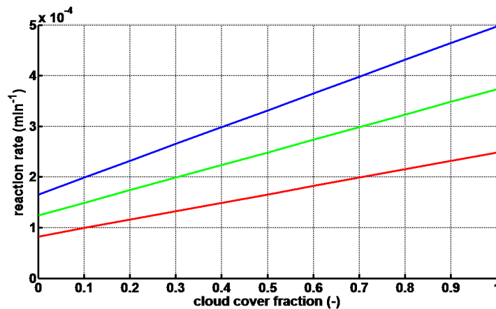
Figure 4-1 reaction rate R_k ( \text{min}^{-1} ) for sulphate formation in clouds, as function of cloud cover fraction, for different values of relative humidity. Red: RH = 90 %, green: RH = 95 %, blue: RH = 100 %.
