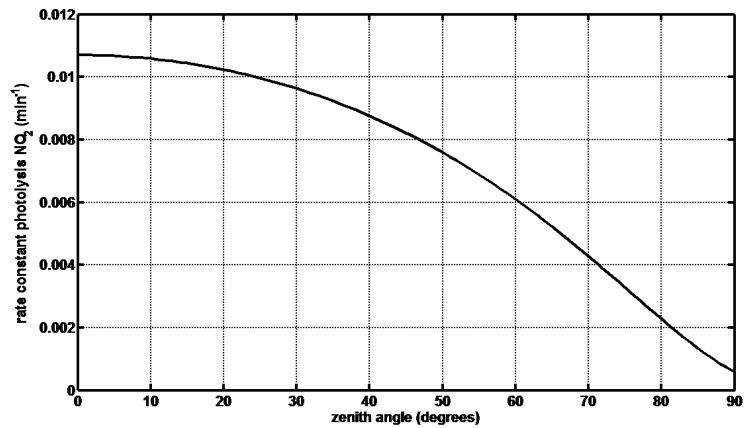
Figure B-1 clear sky reaction rate for the photolysis of NO 2 as function of the solar zenith angle
