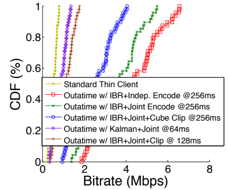
Figure 17: Bandwidth Overhead
