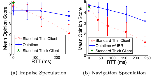
Figure 14: Fable 3 MOS
