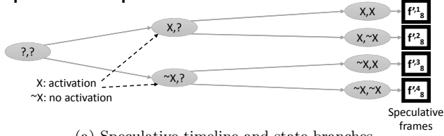
(a) Speculative timeline and state branches
