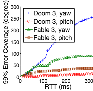
Figure 8: Angular coverage of 99% of prediction errors is much less than 360^\circ even for high RTT.
