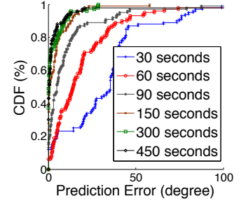
Figure 5: Error Decreases with More Observation Time. Data is for Fable 3 at RTT=160ms.
