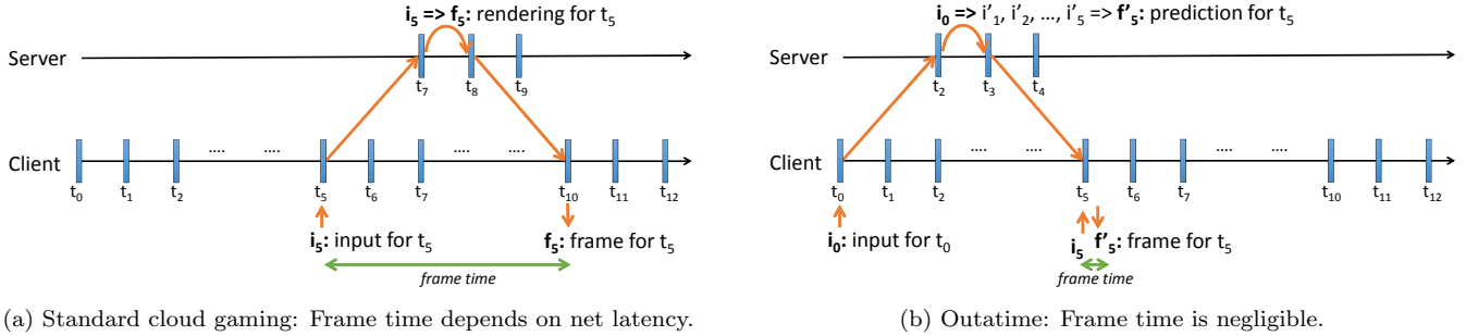
Figure 1: Comparison of frame delivery time lines. RTT= 4 ticks, server processing time = 1 tick.
