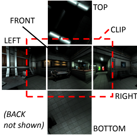
Figure 7: Cube Map Example w/ Doom 3. Clip region shown.
