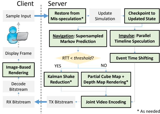
Figure 2: The Outatime Architecture. Bold boxes represent the main areas of this paper’s technical focus.
