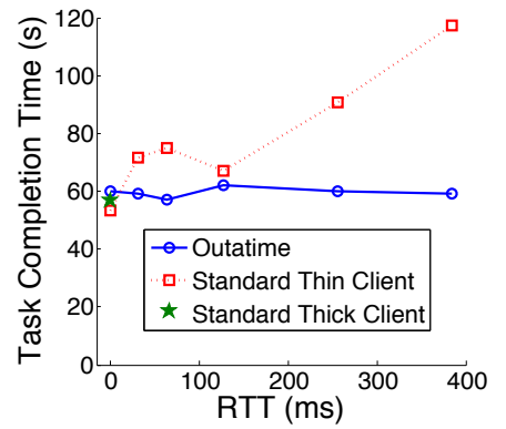
Figure 13: Task Completion Time
