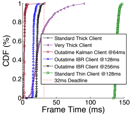
Figure 15: Client Frame Time
