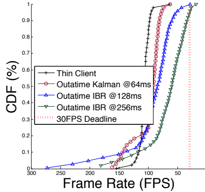
Figure 16: Frame Throughput Measured at Server
