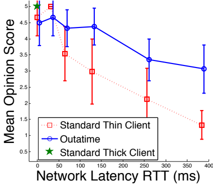
Figure 11: Impact of Latency on User Experience
