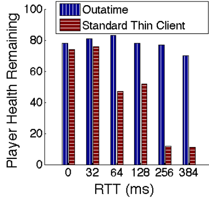
Figure 12: Remaining Health
