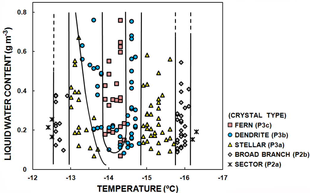
Fig. 2. Habit, temperature, and LWC of each crystal analyzed. The crystals were grown for 10 min.
