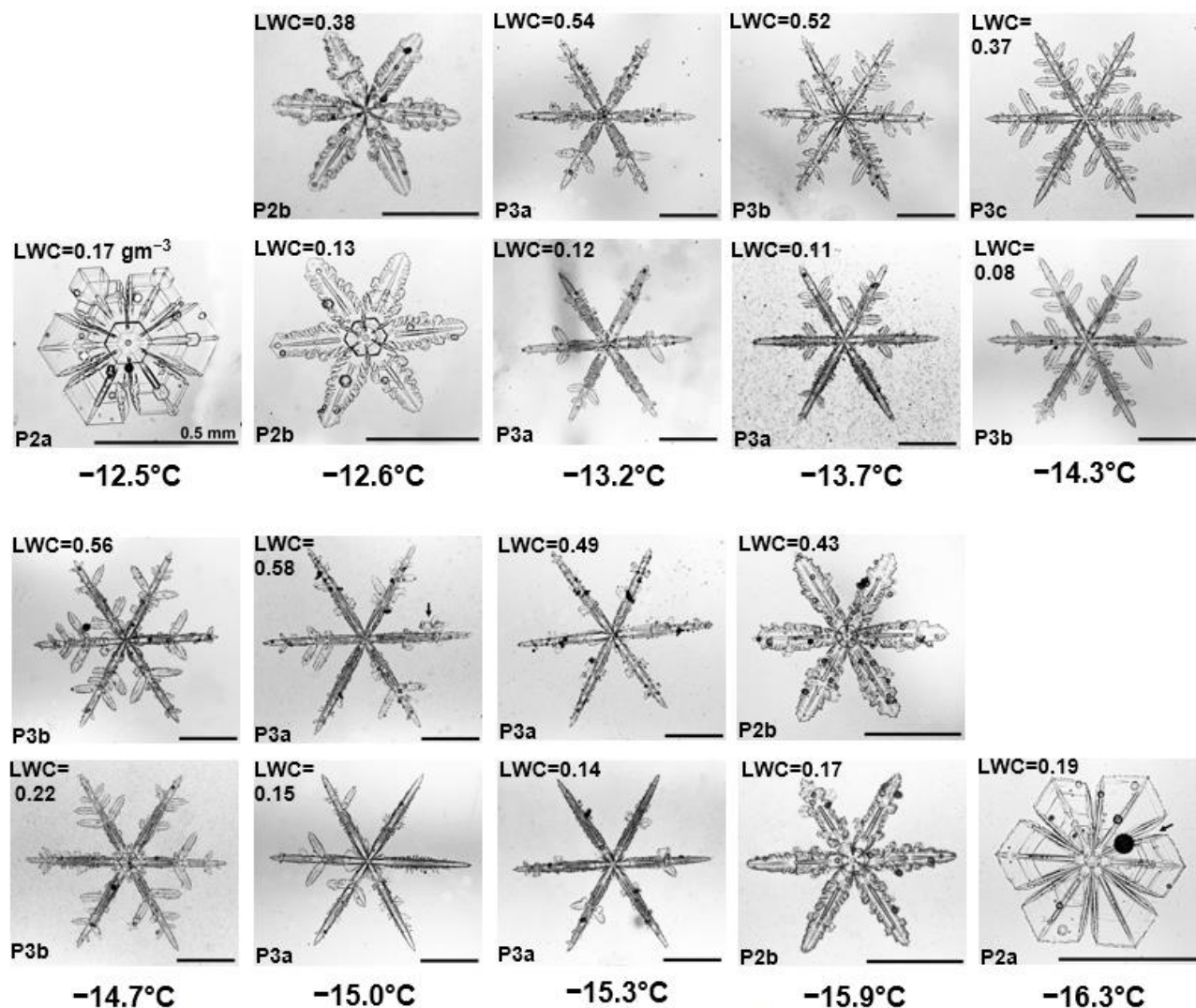
Fig. 1. Variations of crystal shape on temperature after 10 min of growth. At each temperature, a lower photo is for LWCs between 0.08 and 0.22 \text{g m}^{-3} , an upper one is for LWCs between 0.37 and 0.58 \text{g m}^{-3} . The upper and lower left of each crystal shows LWC ( \text{g m}^{-3} ) and the crystal type (see legend, Fig. 2). The arrow in the crystal at -15.0^\circ\text{C} , 0.58 \text{g m}^{-3} marks a spatial dendrite that broke off the mother crystal. Black circles, such as that marked by an arrow at -16.3^\circ\text{C} , are air bubbles in the oil that surrounds the crystals. Scale bar equals 0.5 mm in all images.
