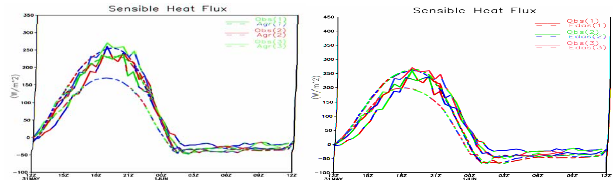
Fig 4: Comparison of sensible heat fluxes (at sites 1,2, and 3) between WRF and IHOP data for simulations initialized AGRMET (left) and EDAS (right).
