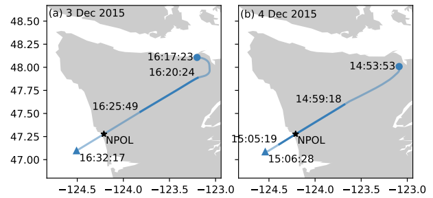
Figure 1. The paths of the flights used in Sect. 5.1 (a) and 5.2 (b). The darker sections of the paths show the flight data used in this study (the rest of the measurements were discarded for the lack of useful data). The time stamps (UTC) denote the beginning and end of each flight and the beginning and end of the data that were used. The gray background shows the outline of the Olympic Peninsula, with Vancouver Island to the north.
