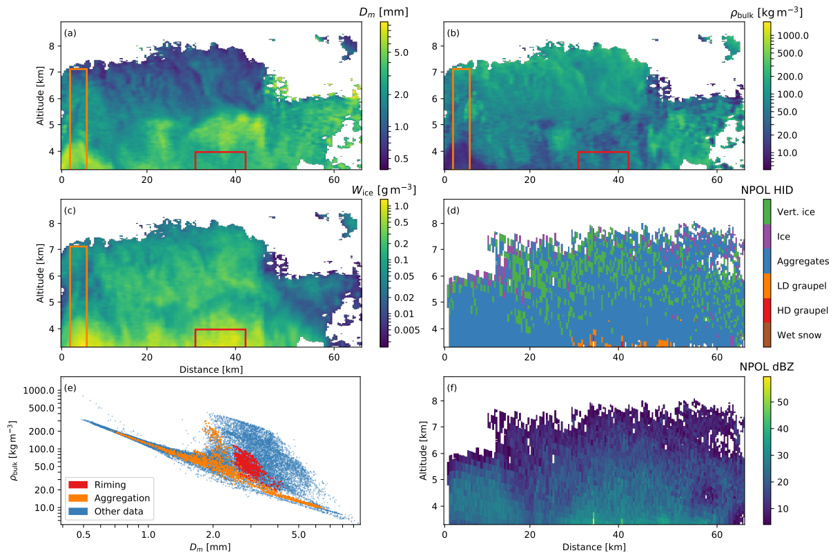
Figure 2. Data from the 3 December 2015 case described in Sect. 5.1. (a) The mass-weighted mean diameter D_m (Eq. 14). (b) The bulk density \rho_{\text{bulk}} (Eq. 16). (c) The ice water content (Eq. 12). (d) The NPOL hydrometeor identification. (e) A scatter plot of D_m and \rho_{\text{bulk}} from (a) and (b), with the red and orange points identifying the data inside the boxes of corresponding colors shown in those panels. (f) The radar reflectivity observed by NPOL.
