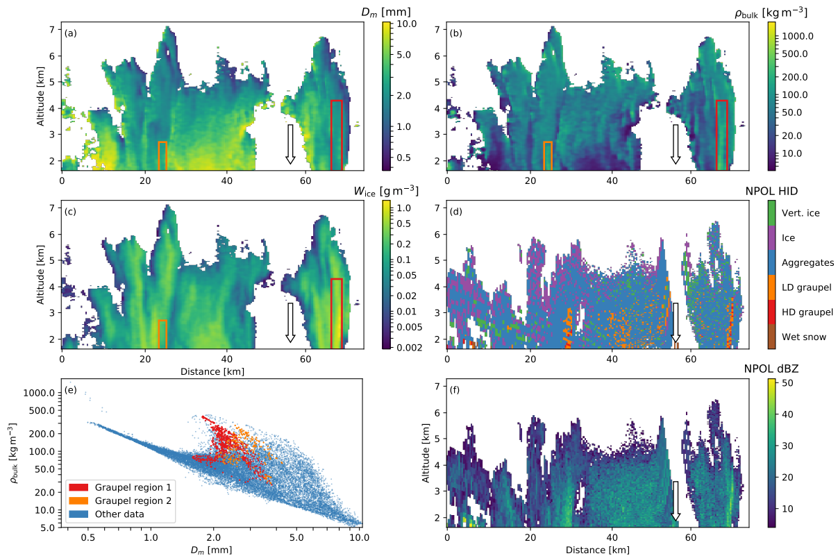
Figure 3. As Fig. 2, except for the 4 December 2015 case described in Sect. 5.2. The location of NPOL on the flight track is marked by the arrow in panels (a)–(d) and (f).
