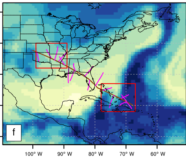
500 hPa refractivity [N units]
