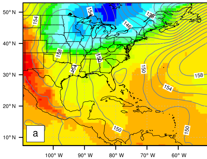
850 hPa temperature [°C]
