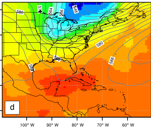
500 hPa temperature [°C]
