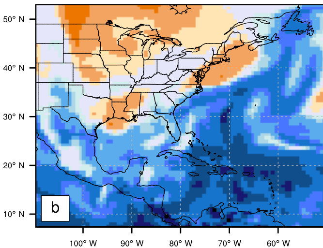
850 hPa mixing ratio [g kg -1 ]
