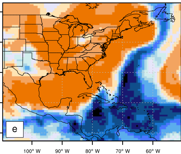
500 hPa mixing ratio [g kg -1 ]
