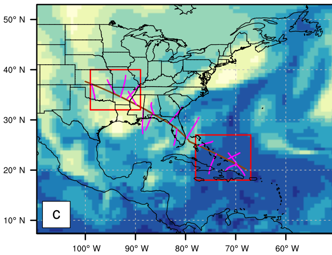
850 hPa refractivity [N units]
