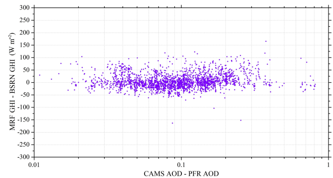
Figure 11. Absolute differences in GHI (in \text{W m}^{-2} ) derived by the MRF technique from the ground-based measurements at Izaña (BSRN pyranometer), as a function of differences in AOD from CAMS and PFR.
