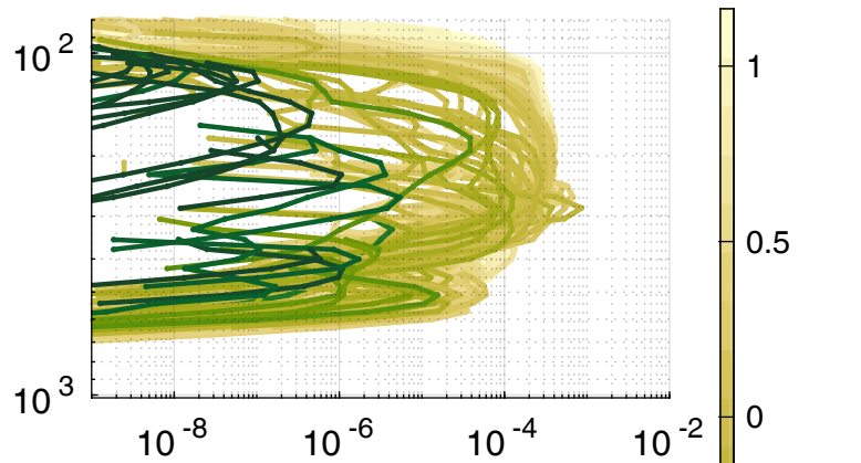
Snow water content
