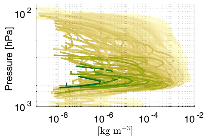
Graupel water content
