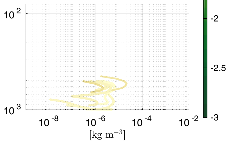
Hail water content
