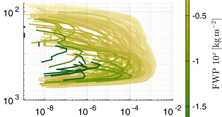
Hail water content
