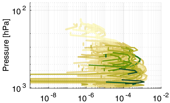
Rain water content
