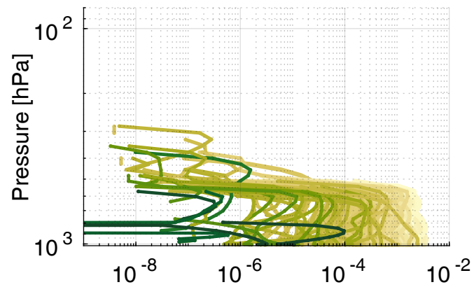
Graupel water content
