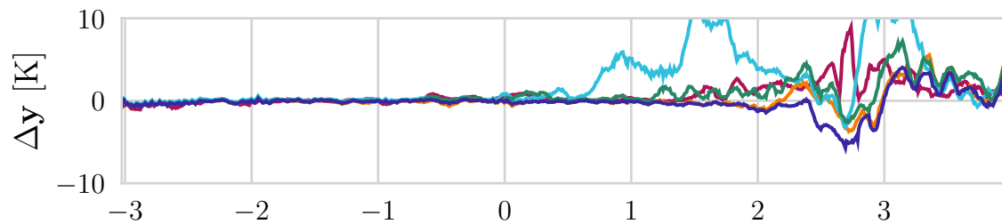
(g) First scene, 664 \pm 4.2 GHz
