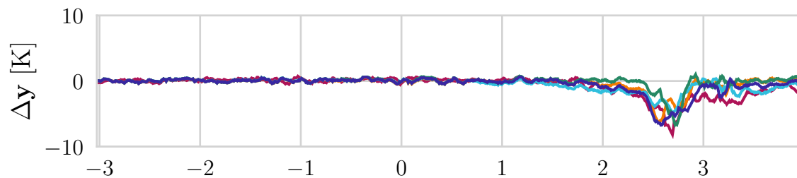
(e) First scene, 325.15 \pm 3.5 GHz
