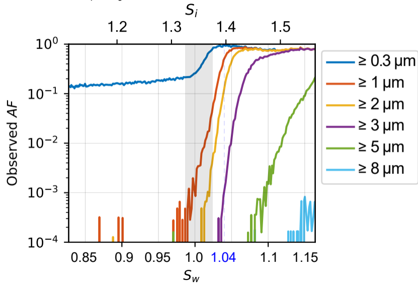
(a) ZRH, \text{NH}_4\text{NO}_3 , 200 nm, 242.9 K, \tau = 9.1 s (965 hPa)
