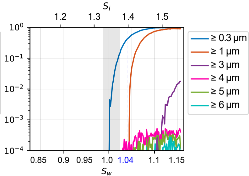
(b) JFJ ambient air, 242.9 K, \tau = 6.1 s (645 hPa)
