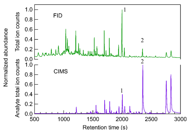
Figure 2. Comparison of chromatograms between FID and CIMS from particle sample generated from limonene–O 3 reaction. The time-series signals of CIMS are the analyte total ion counts, which are the summation of all ions with the reagent ions removed, while signals of FID are single channel. The signals of both CIMS and FID are normalized to the highest peak in the chromatogram.
