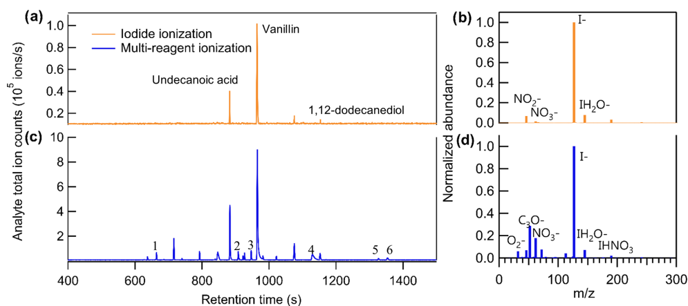
Figure 4. Comparison of chromatograms of analyte total ion counts between (a) iodide ionization and (c) multi-reagent ionization. Comparison of background mass spectra between (b) iodide ionization and (d) multi-reagent ionization. The sample introduced in this run is the mixture of liquid chemical standards and six commercially available fragrances.
