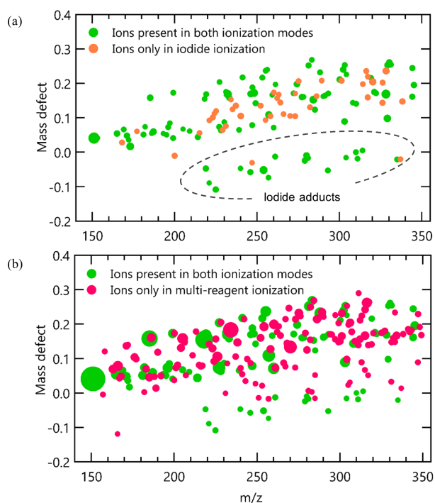
Figure 5. High-resolution mass defect spectrum obtained for liquid mixture samples in (a) iodide ionization mode and (b) multi-reagent ionization mode. The area of markers is proportional to the ion abundance.
