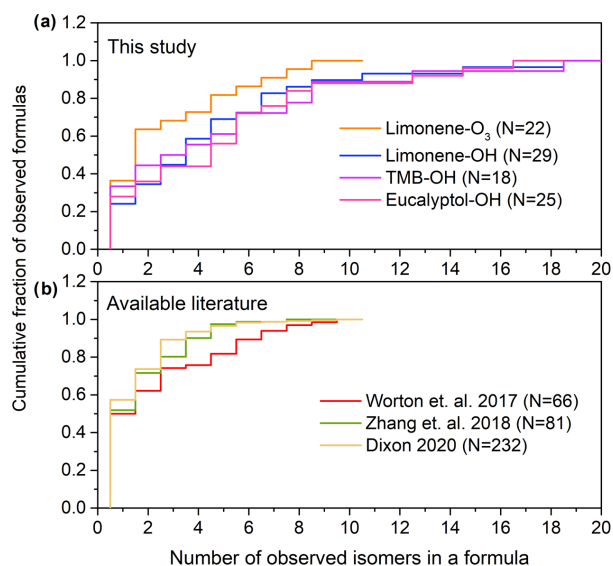
Figure 3. Number of isomers per chemical formula in (a) observed in this work in oxidation experiments and (b) available literature. Data in (b) are from ambient atmospheres in a ponderosa pine forest in California measured by two-dimensional GC without derivatization (Worton et al., 2017), southeastern USA by two-dimensional GC with derivatization (Zhang et al., 2018), and combined datasets from SOA formation measured by liquid chromatography (Bryant et al., 2019; Dixon, 2020). The number, N , of formulas observed in each dataset is provided in the legend.
