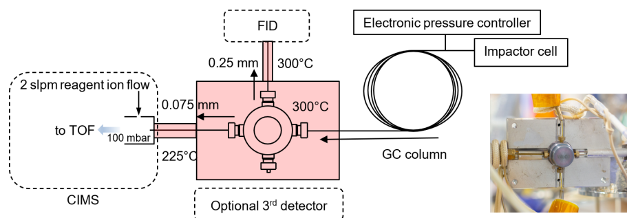
Figure 1. Schematic of the TAG CIMS/FID interface, with a photo inserted. Details of each instrument are simplified. Restrictive capillaries to each detector are used to balance flows to each detector due to differences in pressure (dimensions and temperatures shown).
