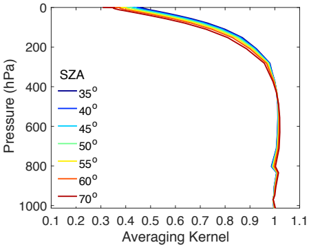
(a) CO 2
