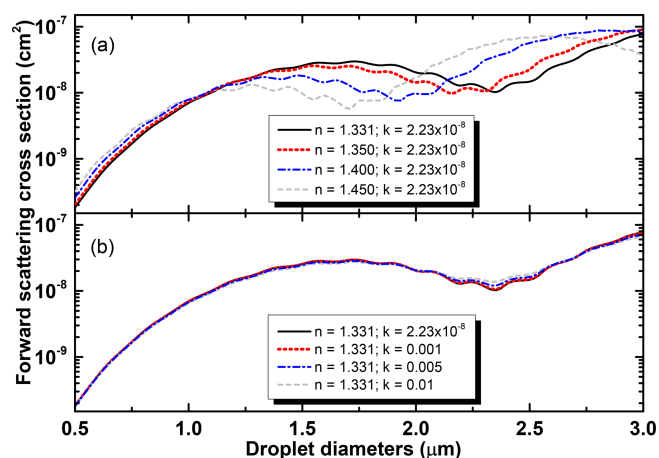
Figure 9. Enlarged view of the small-diameter range of the diagrams of Fig. 8, with focus on the sub-3 \mu\text{m} region. (a) Horizontal shifts no larger than 100 nm may occur when the real part of the refractive index varies. (b) Wide variations in absorption (imaginary part of the refractive index) make almost no changes in the zoomed region of the FWSCS diagrams.
