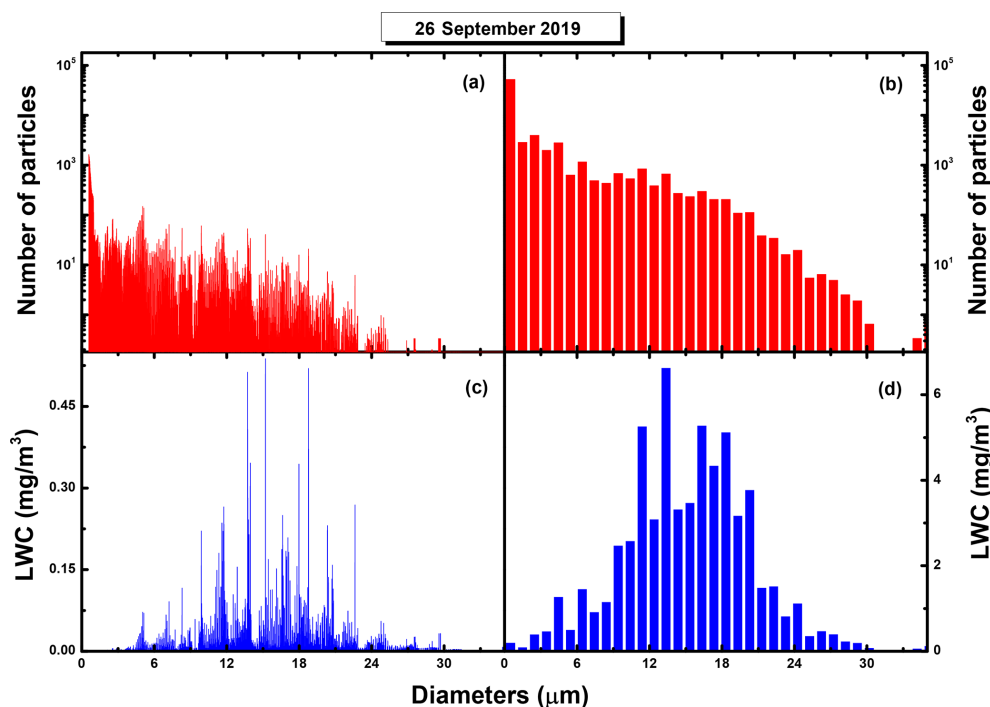
Figure 3. Number (a, b) and LWC (c, d) size distributions obtained from the post-flight analysis of PbP data recorded during a flight line performed on 26 September 2019, over some area of Romania. The diagrams (a) and (c) are detailed distributions and show a fine structure of size modes, which are “wiped” out if spread over coarser size grids, as seen on the histograms (b) and (d) constructed over a structure of 50 equal size bins. Nevertheless, these coarser representations allow for sufficient resolution to accurately compute various averages and are more convenient in evaluating maximal relative errors, as described in the next section. Note the unusual range of LWC values due to the small amounts of liquid water counted in each division of the very fine grid of diameter values. Also, in panel (d), note that the levels of the LWC distribution are higher than those of panel (c) as they collect the contributions of particles from larger divisions of diameter values.
