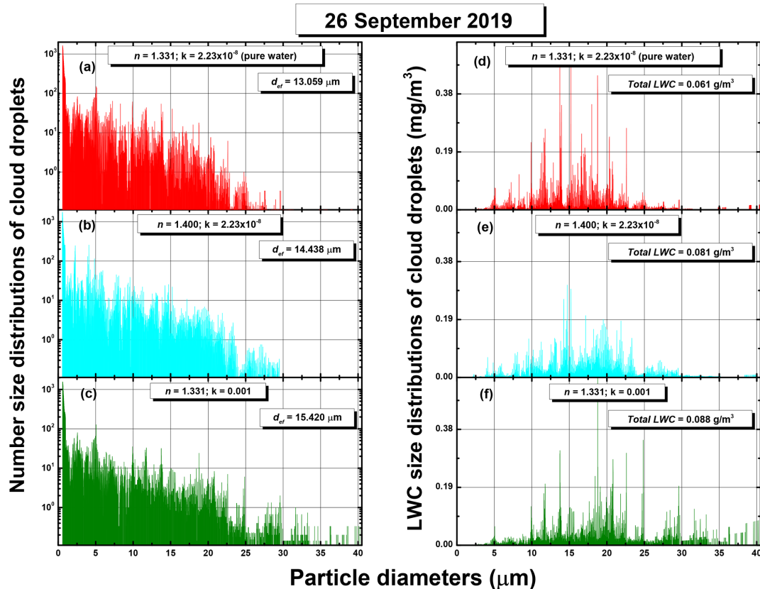
Figure 10. Effect of eventual variations in the refractive index on the detailed number (a–c) and LWC (d–f) size distributions illustrated on data collected in a flight line performed on 26 September 2019, over some part of Romania. Panels (a) and (d) are constructed using the refractive index of pure water. Both distributions shift to the right when either the refractivity (b, e) or the absorption (c, f) increase, indicating that using optical parameters of pure water leads to underestimations in both size and LWC. While the effective diameter, indicated in panels (a)–(c), is underestimated with 10 % to 15 %, the underestimation of the total LWC, indicated in panels (d)–(f), runs between 25 % and 30 % when assuming optical parameters of pure water for contaminated droplets.
