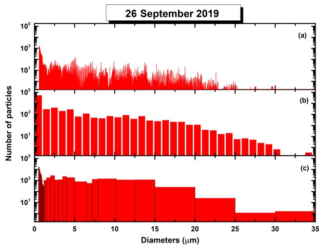
Figure 4. Droplet size distribution of Fig. 3a and b (panels a and b, respectively) shown in comparison with the size distribution of the same droplets constructed over the 30-bin structure used for the in-flight data acquisition.
