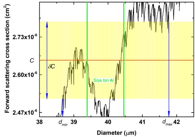
Figure 5. Detail of the FWSCS-diameter diagram showing a measured value, C (red line), of a particle’s FWSCS and the ensuing error strip (yellow region). The particle’s contribution to the distorted size distribution can be computed by considering the “length” of the “blurred” intersection of the error strip with the FWSCS diagram. That length, \Phi_{err} , is defined as the absolute values of the sum of the ordinate projections of all the monotonic parts of the diagram that fit within the error strip. If we further restrict to the part of the curve that fits within the error strip and in the size bin \#i , then the analogous length \Phi_{err}^i results. Its ratio to \Phi_{err} is the weight with which the given particle contributes to the size bin \#i (enclosed by the vertical green lines).
