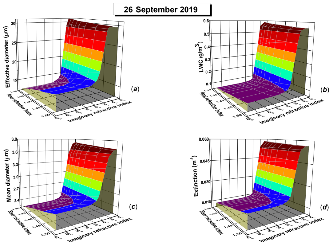
Figure 11. Effective diameter (a), total LWC (b), mean diameter (c) and extinction coefficient computed with the data used to construct Fig. 3b for which the droplet sizing has been performed by assuming the particles have various values of the real and imaginary parts of the refractive index. Each diagram shows a steep increase for imaginary (absorption) index larger than about 0.001, which suggests that droplet sizing is largely underestimated in clouds contaminated with substances that highly absorb the wavelength of the CAS laser.
