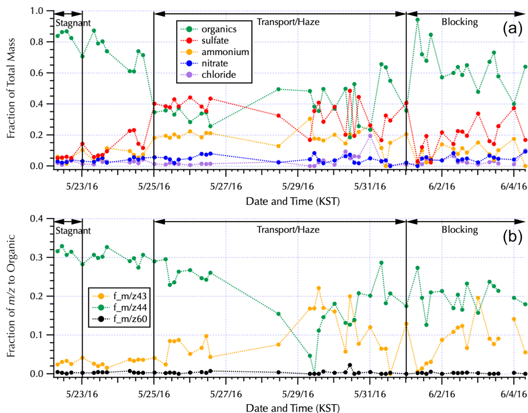
Figure 3. The fraction contributed to the total mass measured by AMS by each of the major aerosol components (a) and the fraction of key water-soluble organic mass fractions to the total AMS organic mass (b) for the complete filter set (Table S1) are shown within the context of the Peterson et al. (2019) meteorological regimes. Note that the long gaps between filters during the Transport/Haze period occurred as the ship transited South Korea's territorial seas with samples obtained when the ship was outside of those waters. The single filter obtained along the south coast (Fig. 1) is the isolated data point on 28 May. The Transport/Haze samples collected from 25–26 May were obtained to the east of the peninsula, and those from 29–31 May were obtained to the west, representing downwind and upwind samples with respect to South Korean emissions and local atmospheric processing, respectively, under the prevalent atmospheric transport of this meteorological period.
