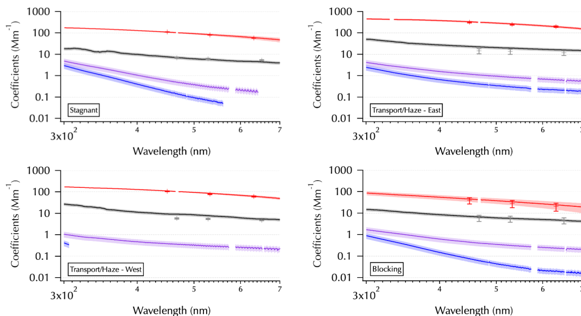
Figure 2. One example from each meteorological regime as shown in Fig. 1 of the spectra set obtained from each filter: mean SpEx \sigma_{\text{ext}} (red line, shaded with \pm 1 SD), \sigma_{\text{abs}} (black line), and \sigma_{\text{MeOH-abs}} and \sigma_{\text{DI-abs}} (purple and blue lines, respectively). Measurement error for all of the absorption coefficient spectra estimated using error propagation (shading, on a log scale this is more difficult to discern for \sigma_{\text{abs}} than for \sigma_{\text{MeOH-abs}} and \sigma_{\text{DI-abs}} ). Mean NT \sigma_{\text{ext}} (red symbols \pm 1 SD) and mean TAP \sigma_{\text{abs}} (gray symbols \pm 1 SD) are shown for comparison. All in units of \text{Mm}^{-1} .
