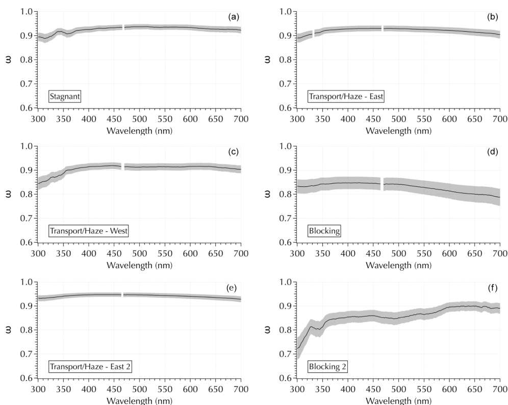
Figure 10. Examples of variability in \omega spectra using the same four examples as in Fig. 2 (a–d), plus an additional example from downwind Transport/Haze and Blocking (e, f, respectively).
