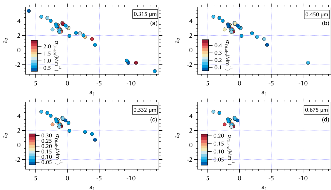
Figure 9. Maps of \sigma_{\text{DI-abs}} ( \text{Mm}^{-1} ) in a_2 vs. a_1 space at 0.315 \mu\text{m} (a), 0.450 \mu\text{m} (b), 0.532 \mu\text{m} (c), and 0.675 \mu\text{m} (d).
