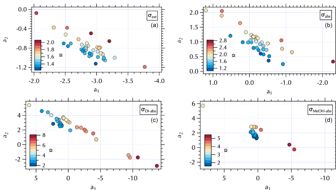
Figure 7. Maps of \alpha in a_2 vs. a_1 space: \sigma_{\text{ext}} (a), \sigma_{\text{abs}} (b), \sigma_{\text{DI-abs}} (c), and \sigma_{\text{MeOH-abs}} (d).
