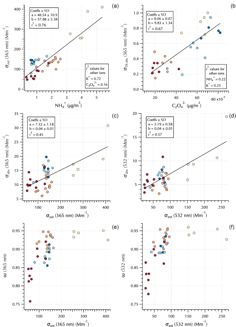
Figure 5. Relationships between 365 nm \sigma_{\text{ext}} and \text{NH}_4^+ (a), 365 nm \sigma_{\text{DI-abs}} and \text{C}_2\text{O}_4^{2-} (b), \sigma_{\text{abs}} and \sigma_{\text{ext}} at 365 and 532 nm (c, d, respectively), and \omega and \sigma_{\text{ext}} at 365 and 532 nm (e, f, respectively). Markers are colored by Peterson et al. (2019) meteorological regime (see Figs. 1 and 4).
