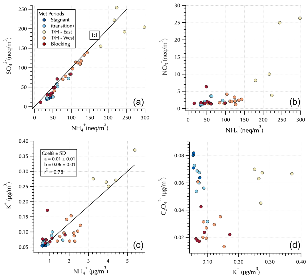
Figure 4. Relationships between \text{SO}_4^{2-} and \text{NH}_4^+ (a) and \text{NO}_3^- and \text{NH}_4^+ (b) in equivalents units and between \text{K}^+ and \text{NH}_4^+ (c) and \text{C}_2\text{O}_4^{2-} and \text{K}^+ (d) in mass units. Markers are colored by Peterson et al. (2019) meteorological regime with the Transport/Haze – East samples downwind of South Korea and the Transport/Haze – West samples upwind of South Korea (see Fig. 1) under the prevailing low-level westerly transport from China during this meteorological regime.
