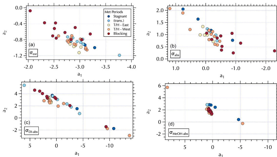
Figure 8. Maps of the meteorological groups as in Fig. 1 in a_2 vs. a_1 space: \sigma_{\text{ext}} (a), \sigma_{\text{abs}} (b), \sigma_{\text{DI-abs}} (c), and \sigma_{\text{MeOH-abs}} (d).
