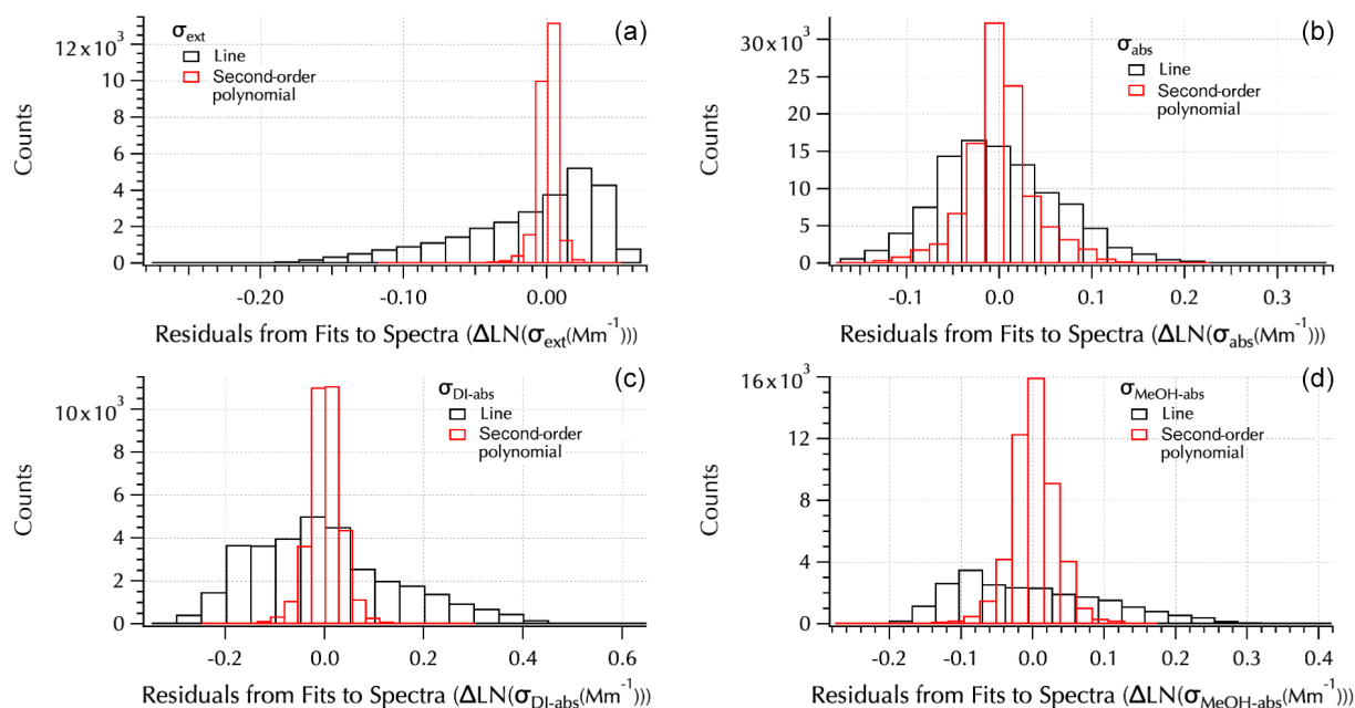
Figure 6. Residuals from linear (black) and second-order polynomial (red) fits to each spectra set: \sigma_{\text{ext}} (a), \sigma_{\text{abs}} (b), \sigma_{\text{DI-abs}} (c), and \sigma_{\text{MeOH-abs}} (d).
