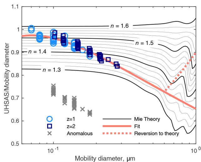
Figure 8. The ratio of apparent to actual diameter measured in the DMA \rightarrow UHSAS tests superimposed on a contour plot of Mie calculations of refractive index and apparent particle diameter. The labels show real refractive indices; absorption is assumed to be 0. The fit line is from Fig. 7, and the dashed line is an arbitrary modification meant to reflect a transition from BB particles in the accumulation mode to sea-salt-like particles at 1 \mu\text{m} . Symbols represent the same data as in Fig. 7.
