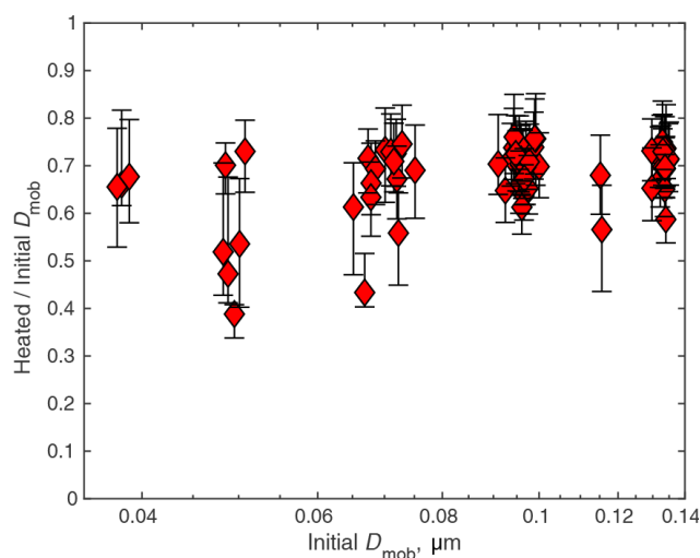
Figure 9. Particle volatility at 300 ^{\circ}\text{C} from the thermal tandem DMA. Symbols are at the median diameter ratio before and after heating. Error bars are the 25th to 75th percentiles, encompassing half of the particles. Data are from all 2018 TDMA measurements in plume (above the MBL and with nephelometer scattering > 20 \text{ Mm}^{-1} ).
