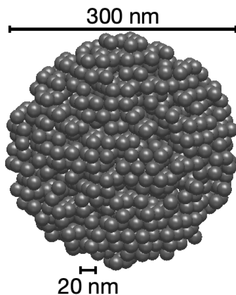
Figure 2. A model 300 nm mobility diameter fullerene soot particle made by packing as many 20 nm spherules as possible into a 320 nm spherical region and then removing random spherules until the mass agreed with the formula in Gysel et al. (2011).
