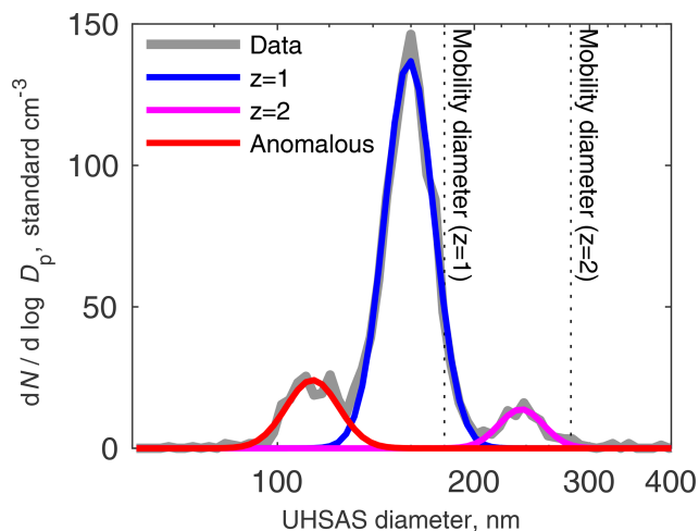
Figure 6. UHSAS size distribution from a DMA selecting 180 nm particles at 1.44° S, 5° E at 1919 m altitude on 23 October 2018 around 14:00 UTC. Colored curves are lognormal fits to the gray data line.
