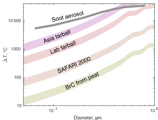
Figure 10. Estimates of particle heating from Eq. (1) for several particle composition types. MSTM was used to find Q_{\text{abs}} for the soot aerosol, while Mie theory was used for the other materials. See Table 1 for the refractive indices used. Shaded regions indicate uncertainty bounds for the accommodation coefficient \alpha ranging from 1 (bottom) to 0.5 (top). The mean free path L was calculated at 700 hPa, near the median pressure during the DMA \rightarrow UHSAS tests. The soot aerosol line uses \alpha = 0.53 , as in Fig. 5, but the lower pressure yields temperatures about 1000 K higher.
