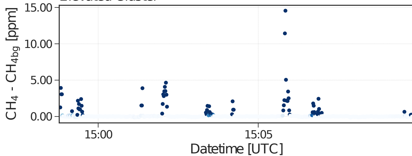
Elevated Cluster
