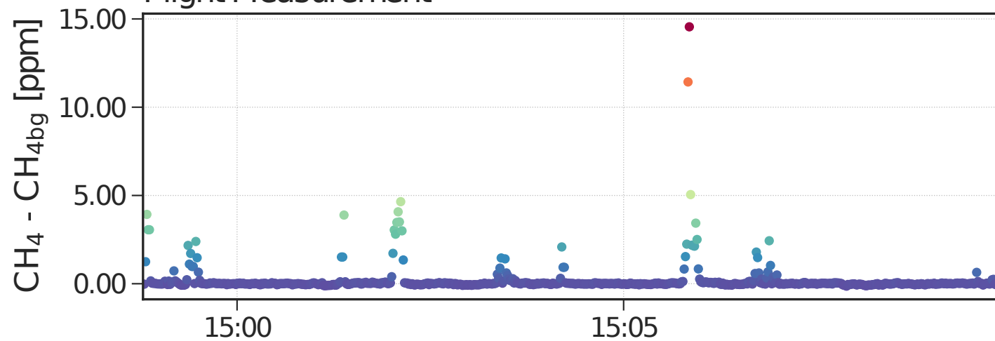
Background Cluster
