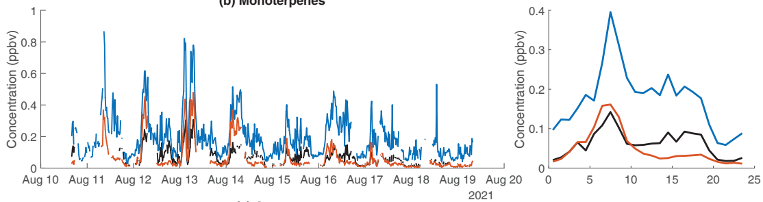
(c) Acetone
