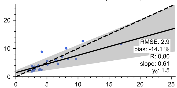
NitroNet vs. AirBase (Italy)
