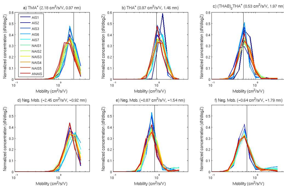
Fig. 3. Examples of mobility standards measurements. Panels (a), (b) and (c) show the response of the ion spectrometers (normalized mobility distribution) for 3 positively charged mobility standards, and panels (d), (e) and (f) for 3 negative mobilities. The black vertical lines represent the mobility that was selected through the HDMA. The mobility and size of the standards are above each plot. TMAI is tetra-methyl ammonium iodide and THAB is tetra-heptyl ammonium bromide.
