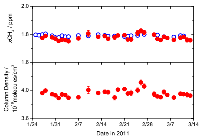
Fig. 8. Time series of column density and x\text{CH}_4 with the standard deviations at JAXA in Tsukuba, Japan. OSA: solid circles (SF = 1.035); FTS: open circles (SF = 0.978).
