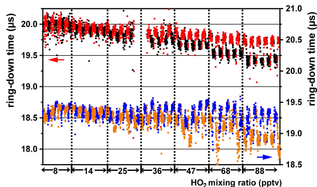
Fig. 11. eCL HO 2 calibration measurement at an inlet pressure of 300 hPa. Left y axis: reactor 1, red – background, black – amplification mode measurement. Right y axis: reactor 2, blue – background, orange – amplification mode measurement. The duration of each HO 2 volume mixing ratio measurement was 10 min.
