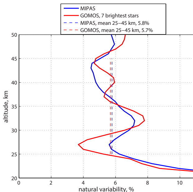
Figure 6. Profiles of natural variability at 20^{\circ} S– 20^{\circ} N in 2008 (Eq. 5) using MIPAS nighttime data and GOMOS data from occultations of seven brightest stars. Vertical dashed lines indicate the mean natural variability over the altitude range 25–45 km.
