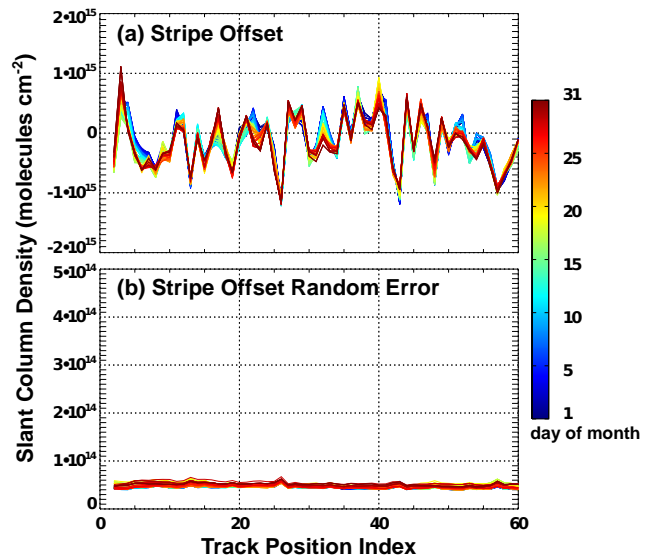
Figure 7. (a) Stripe offset (molecules \text{cm}^{-2} ) derived from a running 5-day mean of the slant columns retrieved over the Sahara ( 20^{\circ} – 30^{\circ} N, 10^{\circ} W– 30^{\circ} E) for July 2006 as a function of cross-track position. Lines are colour coded by day of the month. (b) Estimate of random SCD error (molecules \text{cm}^{-2} ) for (a) induced from noise in the measured radiances.
