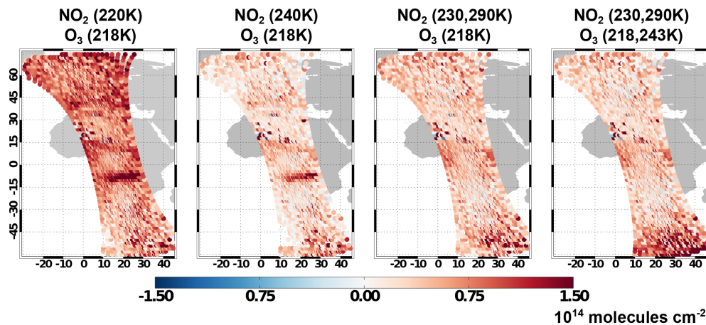
Figure 4. Differences between simulated and true glyoxal slant column densities (molecules cm -2 ) retrieved using NO 2 and O 3 RCSs at different temperatures. Plot titles indicate temperatures of the RCSs used in the retrieval.
