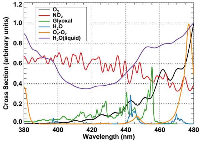
Figure 1. Absorption cross sections for molecules listed in Table 1 degraded to the resolution of OMI. Values have been normalised to order 1 for display purposes.
