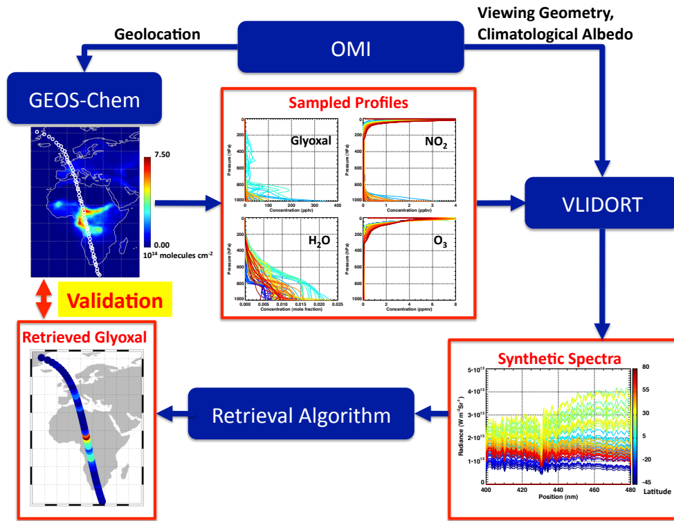
Figure 3. Schematic of the OSSE approach used to optimise the retrieval algorithm.
