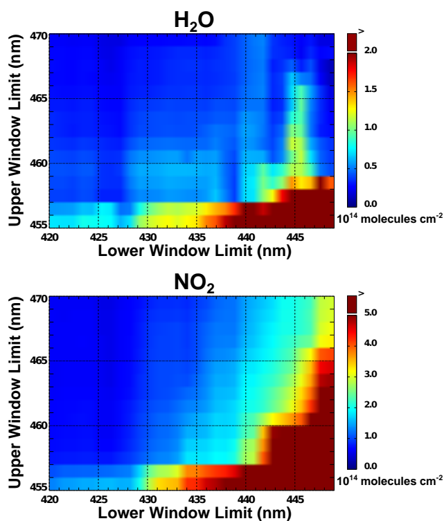
Figure 12. Estimate of mean glyoxal SCD error ( \text{molecules cm}^{-2} ) for all o10430 land pixels due to RCS uncertainties in water vapour (above) and \text{NO}_2 (below).
