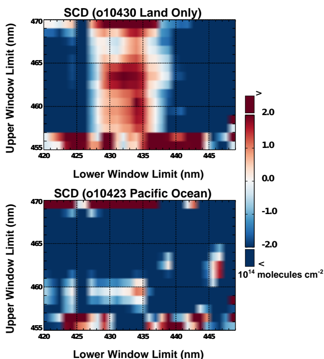
Figure 11. Mean glyoxal Slant column density retrieved as a function of window limits. Top: mean SCD retrieved for all retrievals over land from o10430. Bottom: mean SCD retrieved from 0 to 30° N over the Pacific Ocean (o10423).
