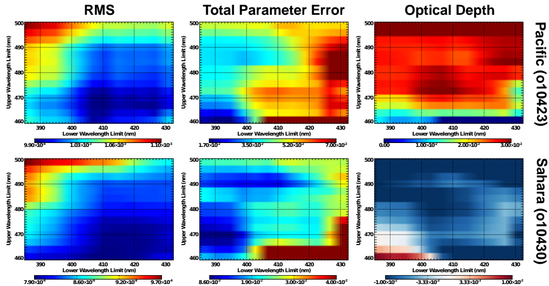
Figure 9. Retrieval window interval maps for spectra over the remote Pacific Ocean (top) and Sahara (bottom). The rms spectrum fit residuals are adjusted for statistical degrees of freedom; cf. Eq. (19). Liquid water optical depths and associated parameter errors are those at 460 nm.
