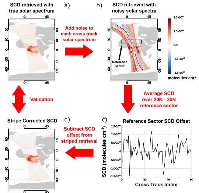
Figure 6. (a) SCD retrieved with true solar spectrum, (b) SCD retrieved with noisy solar spectra, (c) reference sector SCD offset, (d) stripe corrected SCD.
