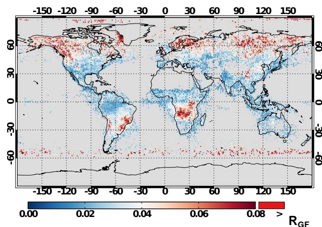
Figure 16. Ratio of glyoxal to formaldehyde VCDs from OMI averaged for June–August 2007.
