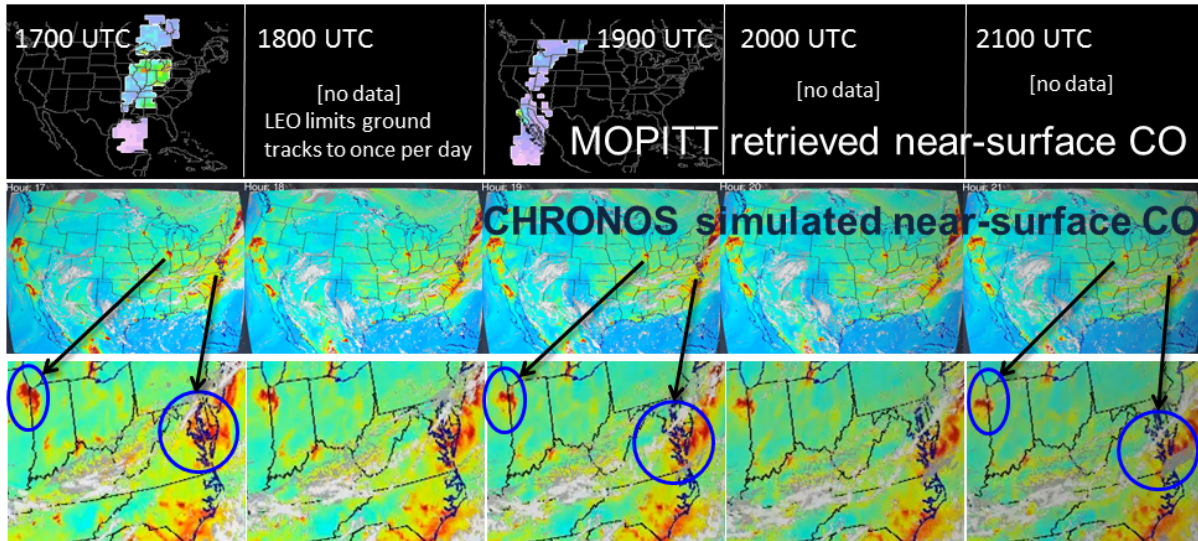
115 Figure 1: Comparison of MOPITT and CHRONOS spatial and temporal coverage over a 5-hour period. The top panels show MOPITT retrievals of near-surface CO for Tuesday Aug. 1, 2006, with pink colors indicating low CO (~ 60 ppbV) and green to red indicating higher values (200 – 300 ppbV). The middle and bottom panels show a simulation of CHRONOS observations using WRF-Chem (Grell et al., 2005) at 4 km horizontal resolution driven by analyzed meteorology (Barth et al., 2012) for the same date. Here blue colors indicate low CO (~60 ppbV), red colors indicate high CO (~300 ppbV) and light greys indicate clouds. Circled areas in the zoomed bottom panels provide detailed examples of changes in CO concentrations over the 5-hour period with pollution from Chicago moving to the west and clouds moving east over the Washington DC area. Urban traffic patterns and weather fronts change the distribution of air pollution throughout the day. Sub-hourly CHRONOS data could assist with attributing the sources of pollution and determining areas affected downwind. 120 125
