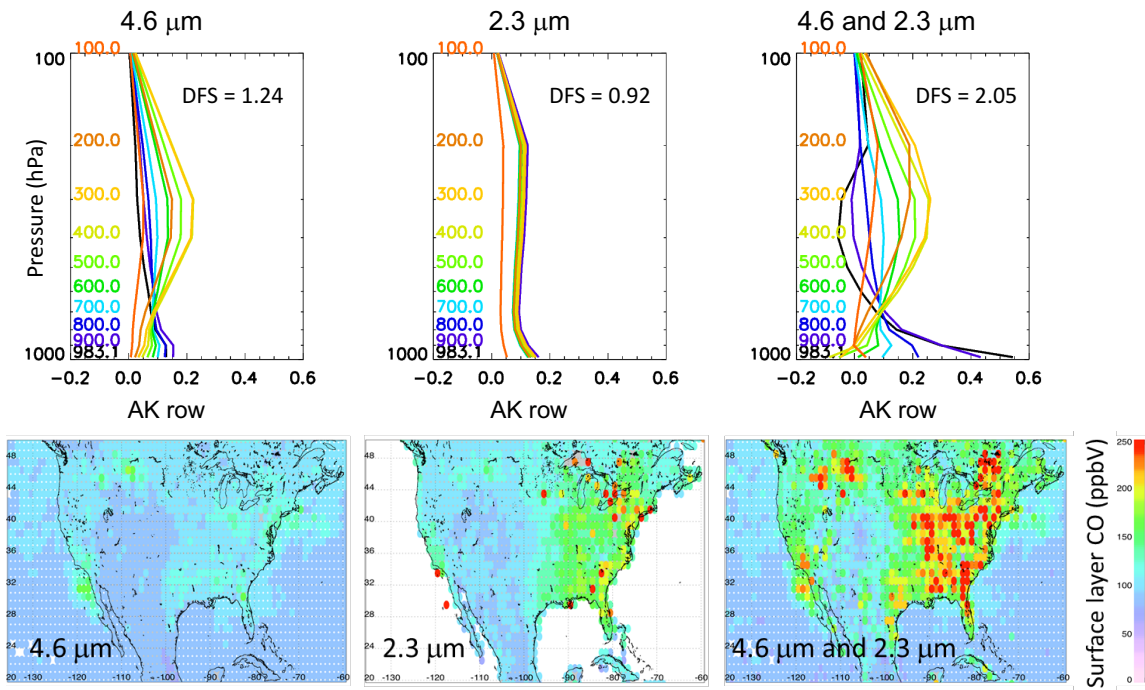
635 Figure 13: Comparison of surface layer CO for MOPITT MWIR (4.6µm), SWIR (2.3 µm) and multispectral (MWIR and SWIR combined) retrievals for Aug. 2000. Top panels show representative averaging kernel (AK) rows, where line colors indicate the pressure layers given on the left side of the panels, for the three retrieval types (location at 30.72°N, 96.50°W). Bottom panels show maps of the surface layer CO abundance indicating how detailed information is 640 obtained in the multispectral retrievals, but is absent in the single channel retrievals.
