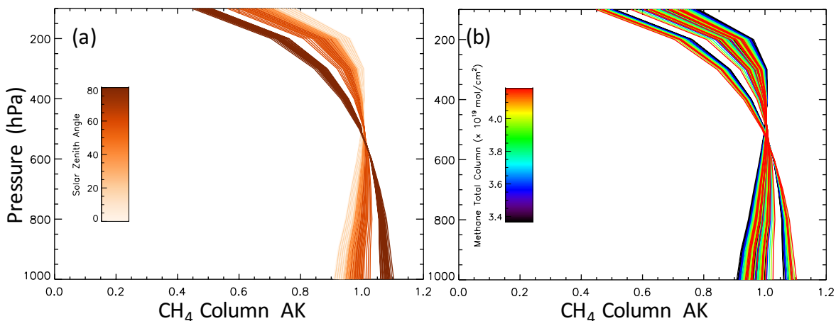
675 Figure 16: Variation of CHRONOS CH 4 averaging kernels for different SZA (left) and CH 4 total column (right) for 100 simulations with different SZA and CH 4 column values. Within each “group” of SZA values, the lesser AK dependence on low-to-high values of CH 4 can be seen.
