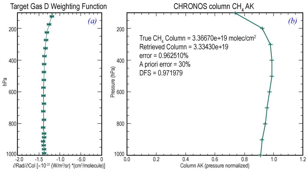
Figure 14: CHRONOS CH 4 D-signal weighting function and retrieval column AK. (a) Sensitivity of the D-signal to changes in CH 4 column ( \partial\text{Rad}(D)/\partial\text{col} ) as a function of vertical pressure for a standard mid-latitude summer atmosphere with albedo = 0.1, SZA = 0°, satellite ZA = 40°. (b) The retrieval column averaging kernel from the corresponding D/A signal ratio and Jacobian. This assumes CHRONOS measurement precision and a priori covariance with 30% diagonal errors and 500 hPa correlation length, (retrieval was performed on a coarser pressure grid than the weighting function calculations). Since the signal source is solar reflectance, the response is nearly uniform vertically with DFS close to 1.
