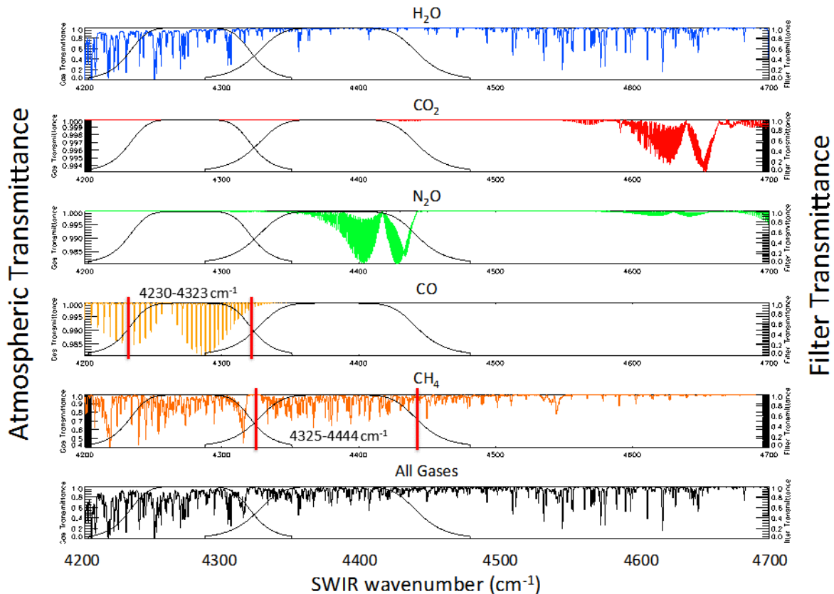
365 Figure 6: Atmospheric transmittance for primary trace gases in the SWIR vs. wavenumber. CHRONOS filter transmission is indicated by smooth bandpass curves with solid red lines at filter half-power points (50% transmittance). CHRONOS measures both CO and CH 4 in the SWIR.
