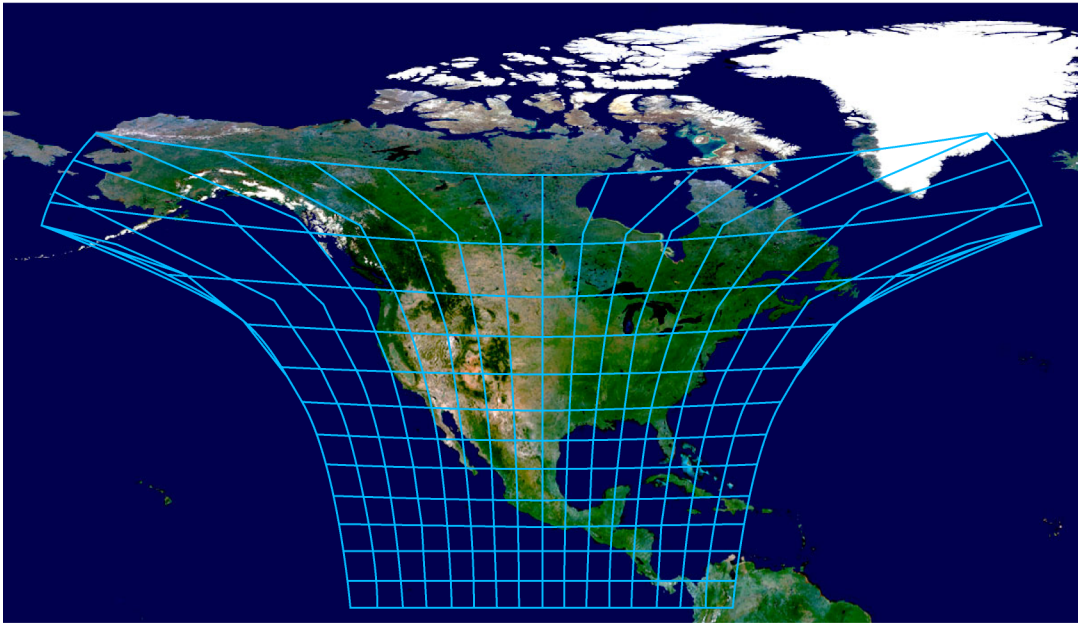
500 Figure 8: CHRONOS field of view from geostationary orbit at 100° W. Each grid cell above represents 125 x 125 pixels. All pixels are acquired with full precision within the ~10 minute CHRONOS data acquisition.
