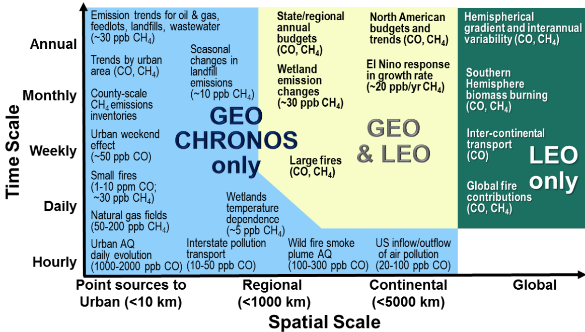
140 Figure 2: CHRONOS’ sub-hourly observations would provide access to the fine temporal and fine spatial scales of CH 4 and CO processes for understanding the emissions and transport of air pollution for air quality, climate, and energy management applications. Estimated abundances are for process contributions above background levels.
