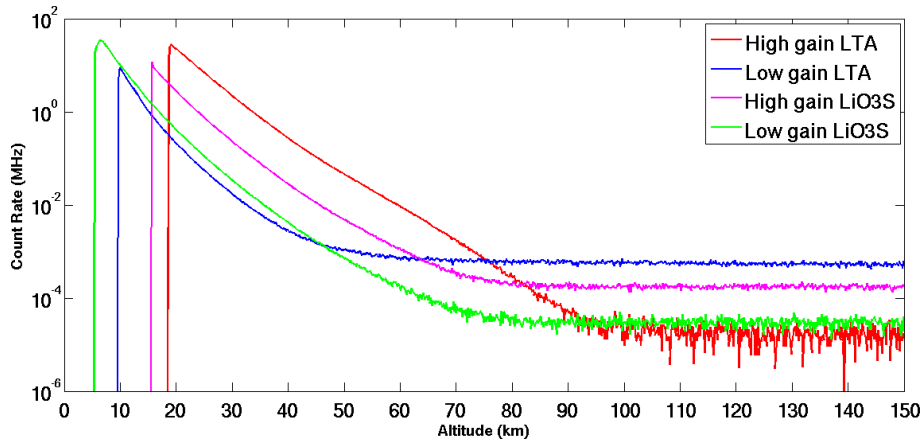
Figure 3: Nightly integrated profiles for high and low gain Rayleigh signals for LTA and LiO 3 S. The background for LTA extends to 246.23 km and for LiO 3 S extends to 154.13 km. A single lidar profile for both LTA and LiO 3 S has a temporal resolution of roughly 2 minutes and 45 seconds and a vertical resolution of 75 m.
