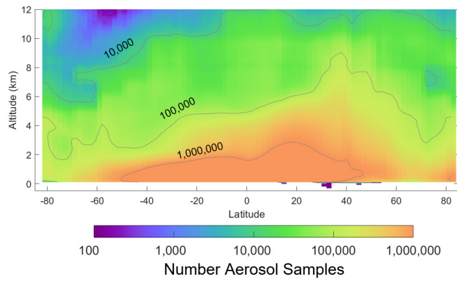
5 Figure 7. Zonal total number of aerosol samples reported by the level 3 product prior to quality screening for 2007–2016 at night, all-sky.
