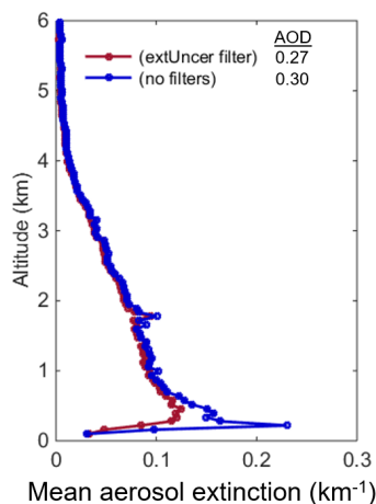
Figure 17. Level 3 \bar{\sigma} with the extinction uncertainty filter (red) and with no filters (blue) over the South America region (Table A1) for 2010 at night, all-sky.
