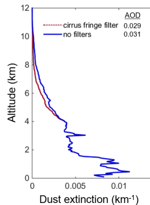
Figure 14. Mean dust extinction with and without cirrus fringe filter for March – May 2010 at night over the Asian dust outflow region [30° N, 60° N; 140° E, 180° E].
