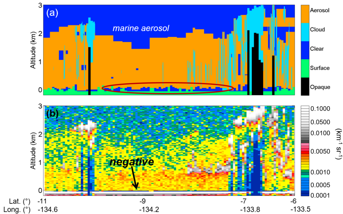
Figure 3. (a) Level 2 feature type classification and (b) level 1B total attenuated backscatter for the granule 2008-08-01T10-17-21ZN passing over the Pacific Ocean. Undetected surface-attached aerosol (circled) and negative attenuated backscatter (arrow) are denoted.
