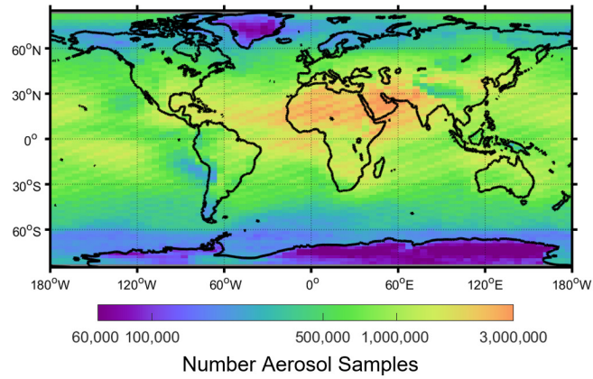
Figure 6. Total number of aerosol samples reported by the level 3 product prior to quality screening for 2007–2016 at night, all-sky.
