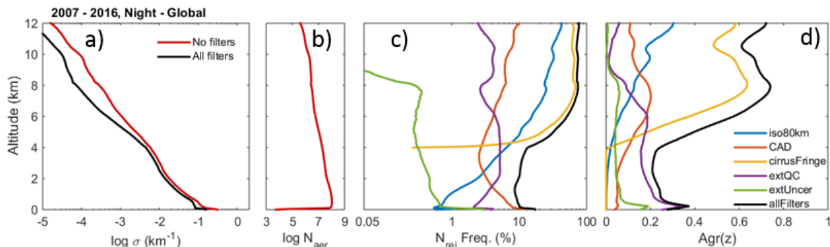
Figure 20. (a) Mean extinction with and without quality filters, (b) number of unfiltered aerosol samples, (c) frequency of aerosol samples rejected, and (d) filter aggressiveness (Eq. (B1)) smoothed vertically over 600 m for 2007–2016 at night, all-sky.
