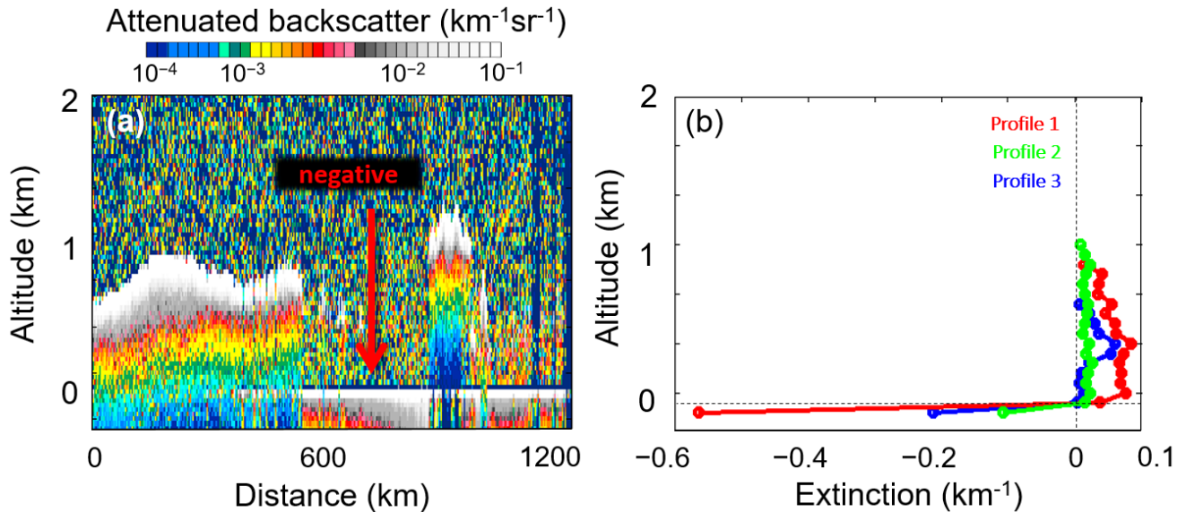
5 Figure 18. Example of NSA in the granule 2006-07-27T00-22-12ZN, centered at \sim 25^\circ S, 10.5^\circ E. (a) Level 1B total attenuated backscatter. (b) Level 2 aerosol extinction profiles.
