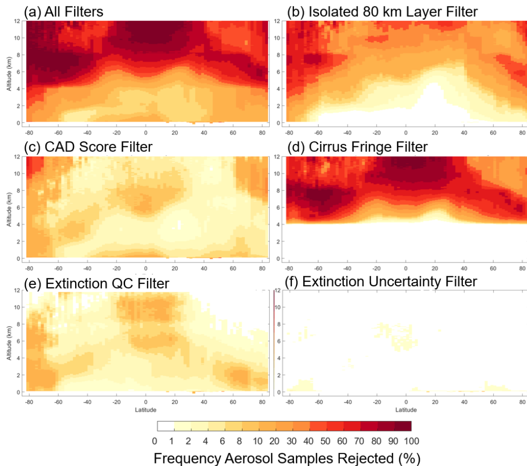
Figure 9. Zonal frequency of aerosol samples rejected by the indicated filter out of all aerosol detected as reported for by the level 3 product for 2007–2016 at night, all-sky.
