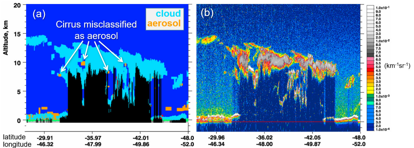
Figure 12. (a) Feature type classification and (b) total attenuated backscatter showing cirrus misclassified as aerosol for the version 3 granule 2011-11-10T03-54-52ZN.
