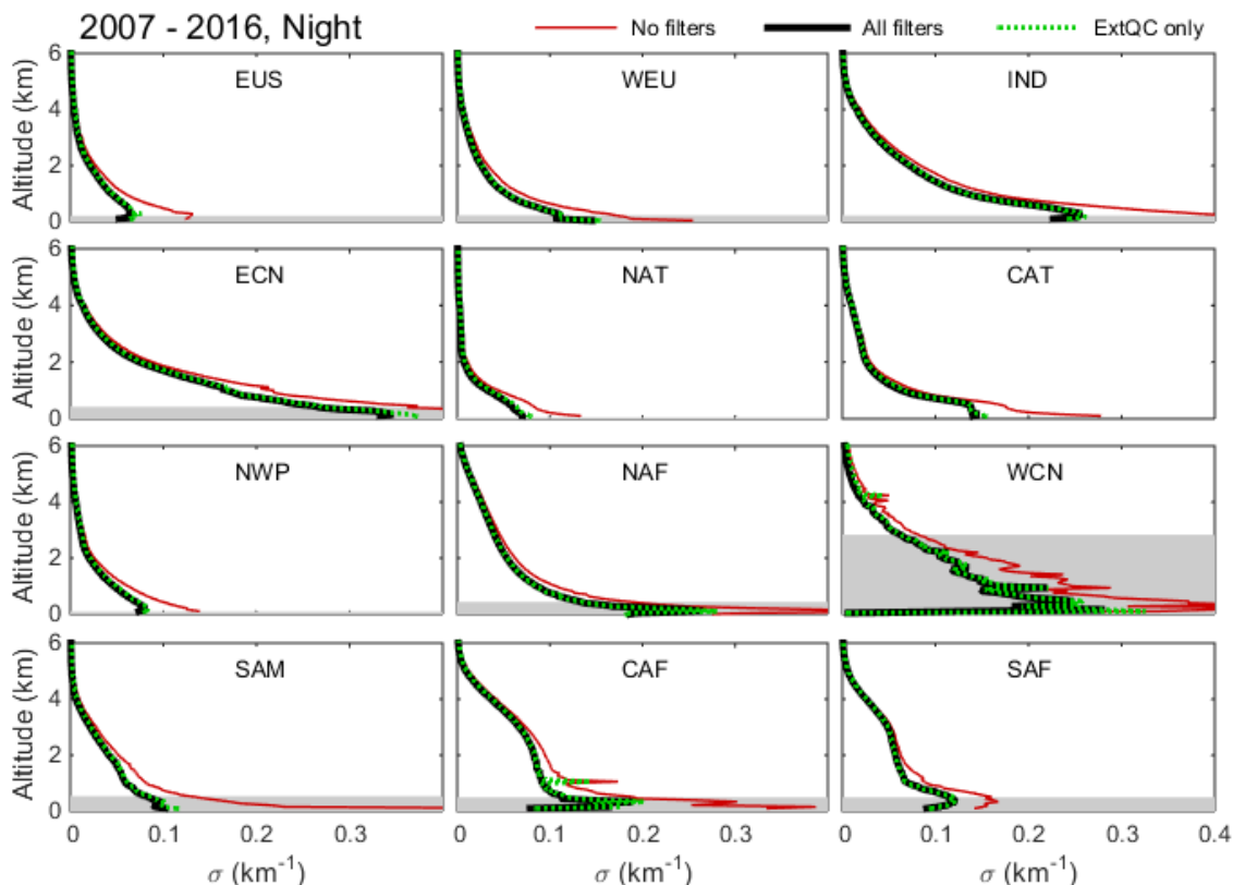
10 Figure 22. Regional \bar{\sigma} with no filters (red), all filters (black), and the extinction QC filter only (green dashed) for 2007–2016 at night, all-sky. The median surface elevation indicated by the shaded grey region.
