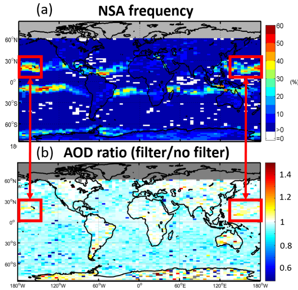
Figure 19. (a) Frequency of level 1B profiles containing the negative signal anomaly (NSA) in parallel 532 nm lidar channel and (b) ratio of level 3 mean AOD with and without NSA mitigation filter for July 2008 at night. Note that the geographic location of enhanced NSA frequency changes seasonally.
