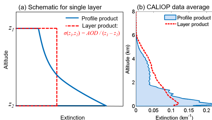
Figure 1. (a) Schematic example of aerosol extinction profile for an individual layer reported by the profile product (blue) and by the layer product (red dashed) where mean aerosol extinction is computed from the layer AOD divided by the geometric depth ( \Delta z ). (b) Seasonal average of CALIOP aerosol extinction computed by the profile product (blue, filled) and by the layer product (red dashed) for JJA 2007 at night over the central Atlantic Ocean region (Table B1).
