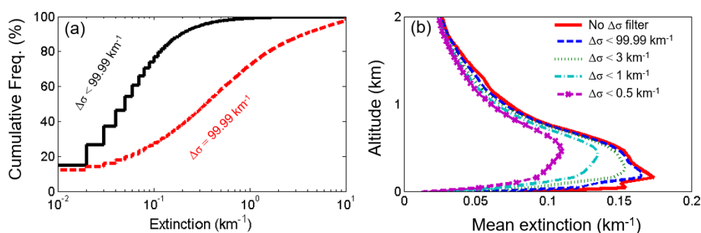
10 Figure 16. (a) Cumulative frequency distributions of level 2 \sigma where \Delta\sigma \neq 99.99 (black) and \Delta\sigma = 99.99 (red) for August 2007; (b) level 3 \bar{\sigma} profiles without the \Delta\sigma filter (red) and with varying upper limits on the \Delta\sigma filter threshold (dashed lines) for mid-Atlantic Ocean, 2007, all-sky at night.
