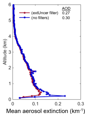
Figure 17. Level 3 \bar{\sigma} with the extinction uncertainty filter (red) and with no filters (blue) over the South America region (Table B1) for 2010 at night, all-sky.
