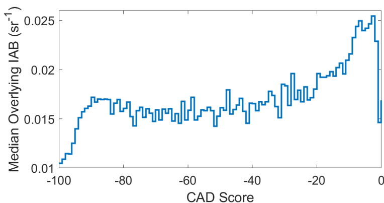
5 Figure 10. Median overlying integrated attenuated backscatter (IAB) for aerosol layers having the indicated CAD score for 2010 at night.
