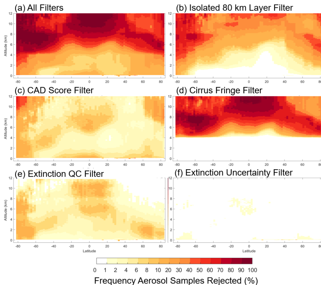
Figure 9. Zonal frequency of aerosol samples rejected by the indicated filter out of all aerosol detected for 2007–2016 at night, all-sky.
