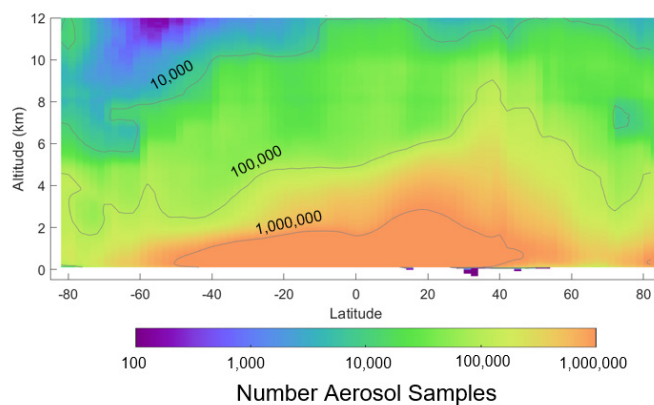
Figure 7. Zonal total number of aerosol samples prior to quality screening for 2007–2016 at night, all-sky.
