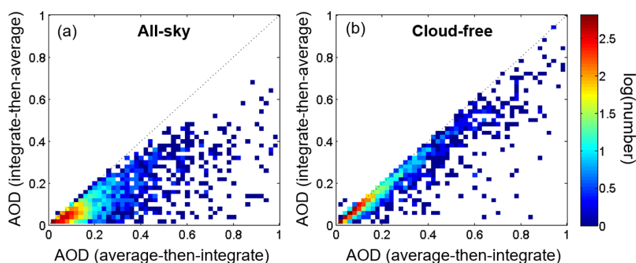
20 Figure 5. Level 3 mean AOD for all latitude/longitude grid cells in July 2007 at night for (a) all-sky and (b) cloud-free sky conditions. Colors represent the number of grid cells on a logarithmic scale.
