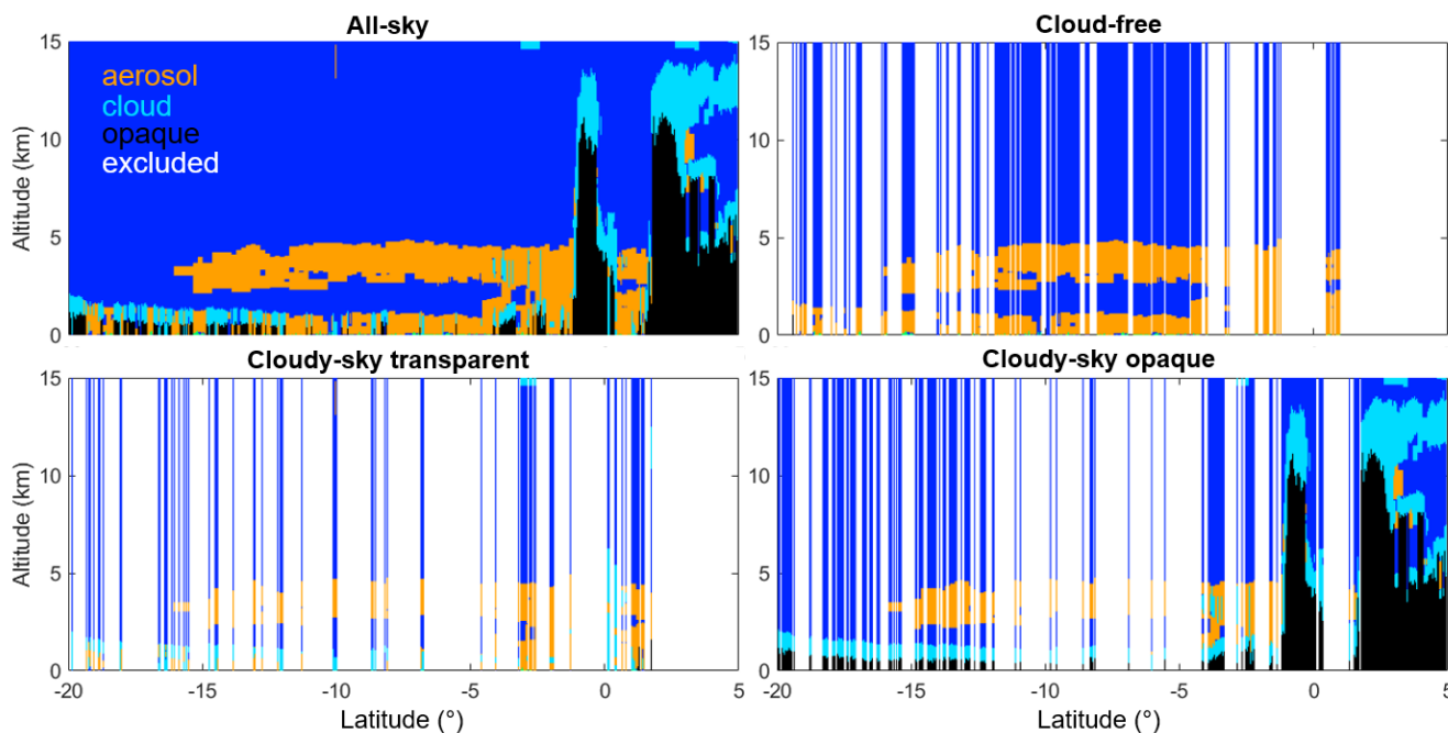
Figure 2. Feature classifications for an individual level 2 granule (2008-01-01T01-30-23Z) demonstrating the four level 3 sky conditions. Data in white columns are excluded for the indicated sky condition. Clouds, aerosols and totally attenuated (opaque) features are light blue, orange, and black, respectively.
