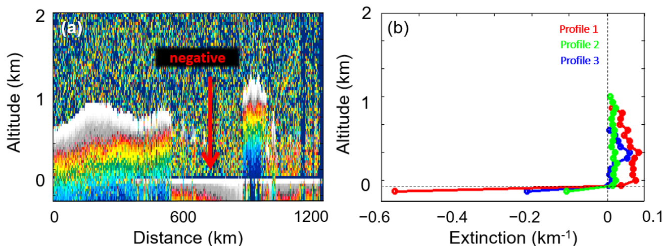
Figure 18. Example of NSA in the granule 2006-07-27T00-22-12ZN, centered at \sim 25^\circ S, 10.5^\circ E. (a) Level 1B total attenuated backscatter. (b) Level 2 aerosol extinction profiles.
