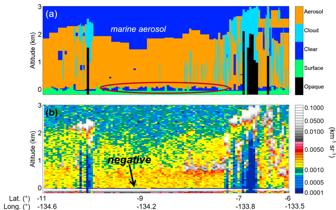
Figure 3. (a) Level 2 feature type classification and (b) level 1B total attenuated backscatter for the granule 2008-08-01T10-17-21Z passing over the Pacific Ocean. Undetected surface-attached aerosol (circled) and negative attenuated backscatter (arrow) are denoted.
