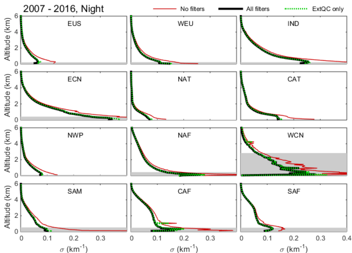
Figure 22. Regional \bar{\sigma} with no filters (red), all filters (black), and extinction QC filter only (green dashed) for 2007–2016 at night, all-sky. The median surface elevation indicated by the shaded grey region.
