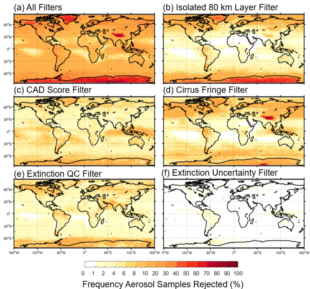
Figure 8. Frequency of aerosol samples rejected by the indicated filter out of all aerosol detected for 2007–2016 at night, all-sky.
