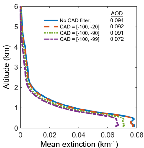
15 Figure 11. Mean extinction without the CAD score filter (blue solid line) and with three different CAD score ranges (dashed lines) for 2010 at night, all-sky, ocean-only, 50° S–50° N.
