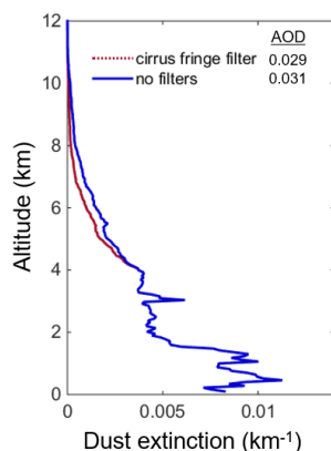
15 Figure 14. Mean dust extinction with and without cirrus fringe filter for MAM 2010 at night over the Asian dust outflow region [30° N, 60° N; 140° E, 180° E].
