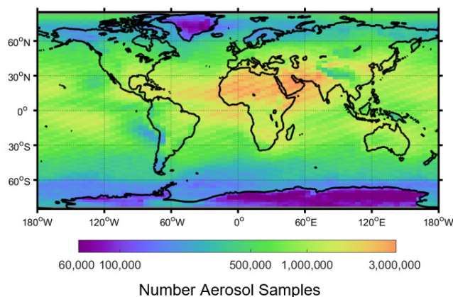
Figure 6. Total number of aerosol samples prior to quality screening for 2007–2016 at night, all-sky.
