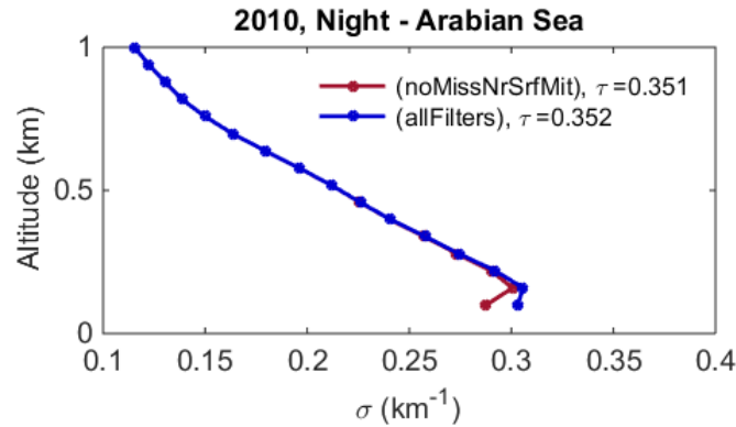
Figure 4. Mean aerosol extinction with (blue) and without (red) undetected near-surface aerosol mitigation over the Arabian Sea [11° N, 27° N; 55° E, 70° E], all-sky 2010 at night.
