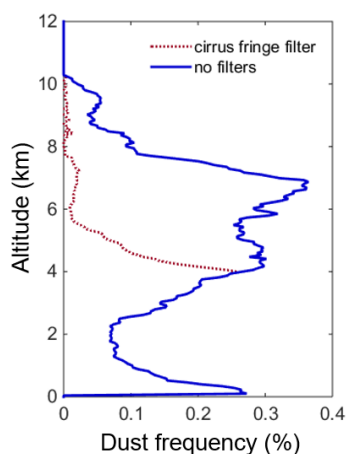
5 Figure 13. Dust detection frequency ( 100 \times N_{dust} / N_{all\ aerosol} ) with and without the cirrus fringe filter for SON 2010 at night over the south Pacific Ocean [30° S, 55° S; 80° W, 180° W].
