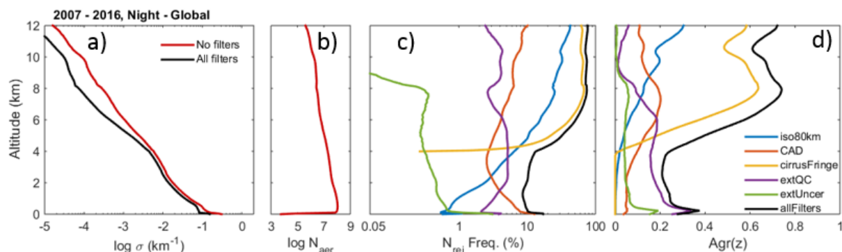
Figure 20. (a) Mean extinction with and without quality filters, (b) number of unfiltered aerosol samples, (c) frequency of aerosol samples rejected, and (d) filter aggressiveness (Eq. (A1)) smoothed vertically over 600 m for 2007–2016 at night, all-sky.
