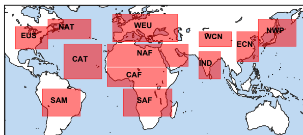
15 Figure 21. Region definitions, similar to those defined by Yu et al. (2010): EUS = Eastern United States, WEU = Western Europe, IND = India, ECN = Eastern China, NAT = North Atlantic Ocean, CAT = Central Atlantic Ocean, NWP = Northwest Pacific Ocean, NAF = North Africa, WCN = Western China, CAF = Central Africa, SAF = Southern Africa. Geographic boundaries are specified in Table B1.
