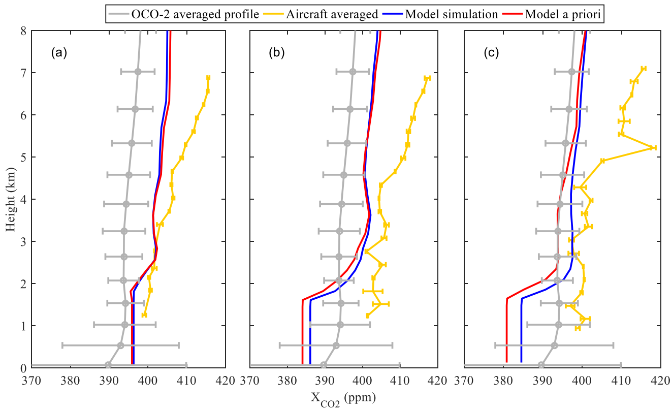
490 Figure 6. Comparison of aircraft measurements (in situ measurement data are shown by the yellow line) with 1 standard deviation (yellow bars) collected on (a) 7, (b) 9, and (c) 10, August Tan-Tracker (v1) data (blue line) and the a priori profile of it (red line) at the location of Jiansanjiang linearly interpolated to the observation times on (a) 7, (b) 9, and (c) 10 August, and the OCO-2 averaged profile (gray line) for the aircraft flight area from 5 August with 1 standard deviation (grey bars).
