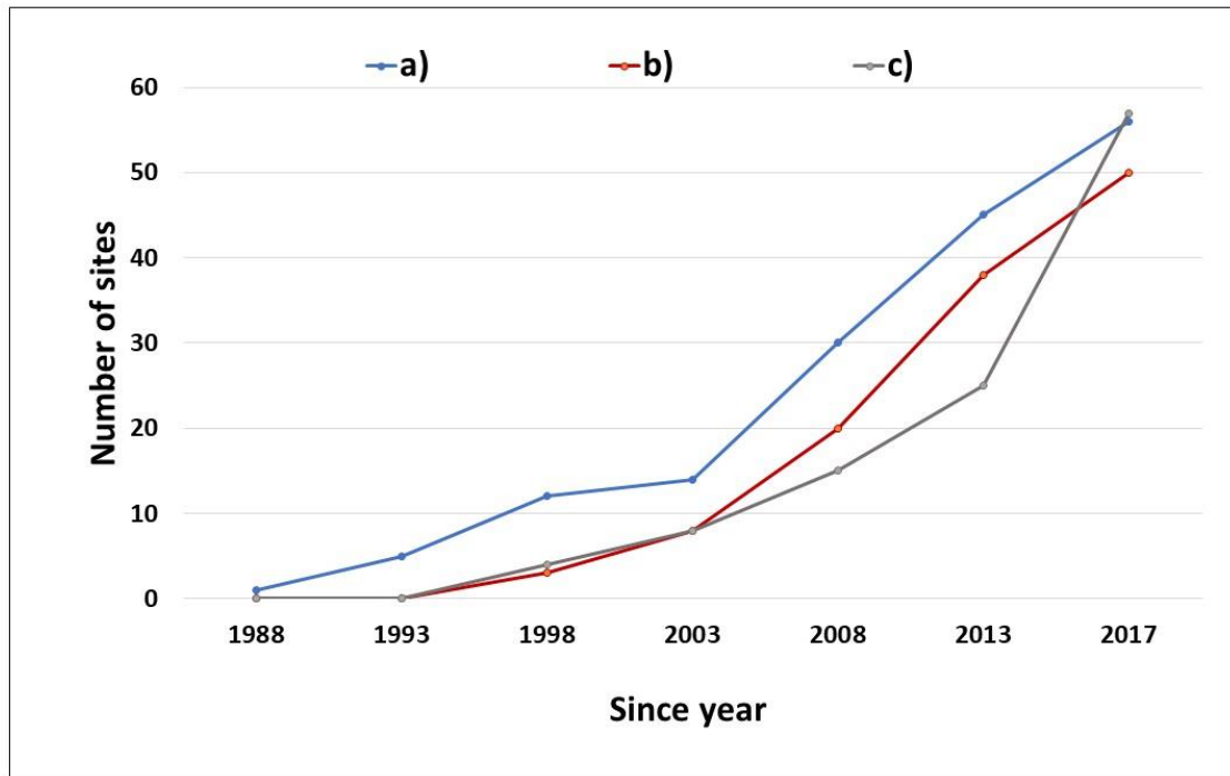
Figure 3: Cumulative number of sites providing information to WDCA for the aerosol variables: a) scattering, b) absorption and c) combined size and particle number concentration.
