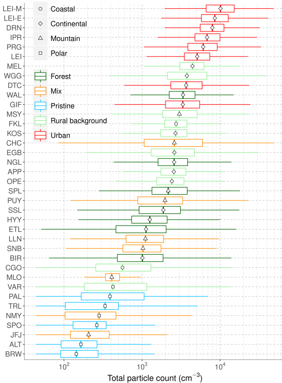
Figure 8 : Yearly median of the total particle number concentration ( N_{tot} ). The markers represent the median of the data and the lower and upper edges of the box indicate the 25th and 75th percentiles, respectively. The length of the whiskers represents 1.5 interquartile range. Different markers and box colors indicate geographical categories and footprint, respectively, according to Table 3. Note that only the sites with sufficient annual coverage (i.e. >75%) are presented
