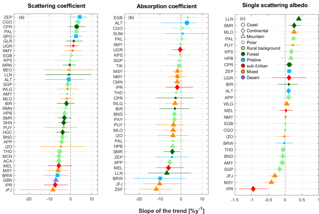
Figure 11: Annual trends for (a) the scattering coefficient, (b) the absorption coefficient and (c) the single scattering albedo derived for SARGAN stations providing 10yr time series ending in 2016-2018. The larger symbols represent statistically significant trends at 95% significance level derived from the Mann-Kendall seasonal test (Collaud Coen et al., 2020). The lines are the 90% confidence limit upper and lower confidence limits derived from the Sen's slope estimator.
