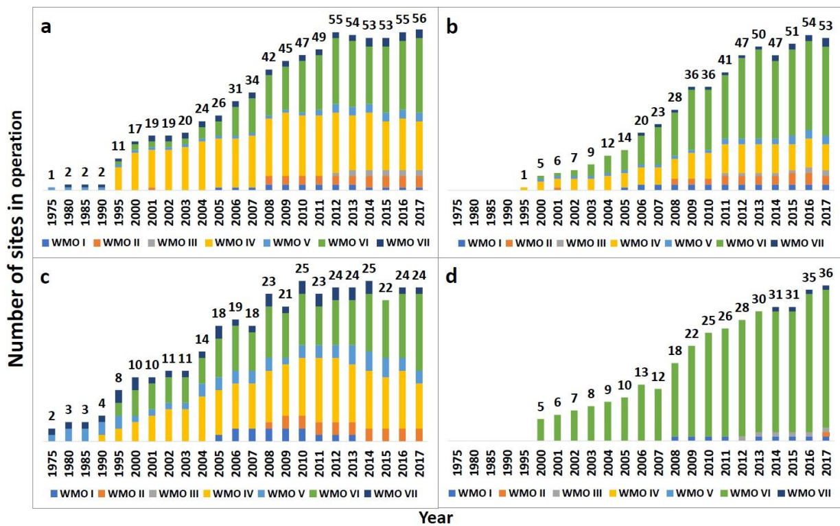
1970 Figure 2: The evolution of data provision in SARGAN for optical (panel a, b), and physical parameters split between sites providing particle number concentration (panel c) and sites providing Particle Number size distribution (panel d) over the period 1975-2017 for the WMO regions. WMO I = Africa, WMO II = Asia, WMO III = South America, WMO IV = North America, Central America and the Caribbean, WMO V = the South-West Pacific, WMO VI = Europe, WMO VII = Polar
