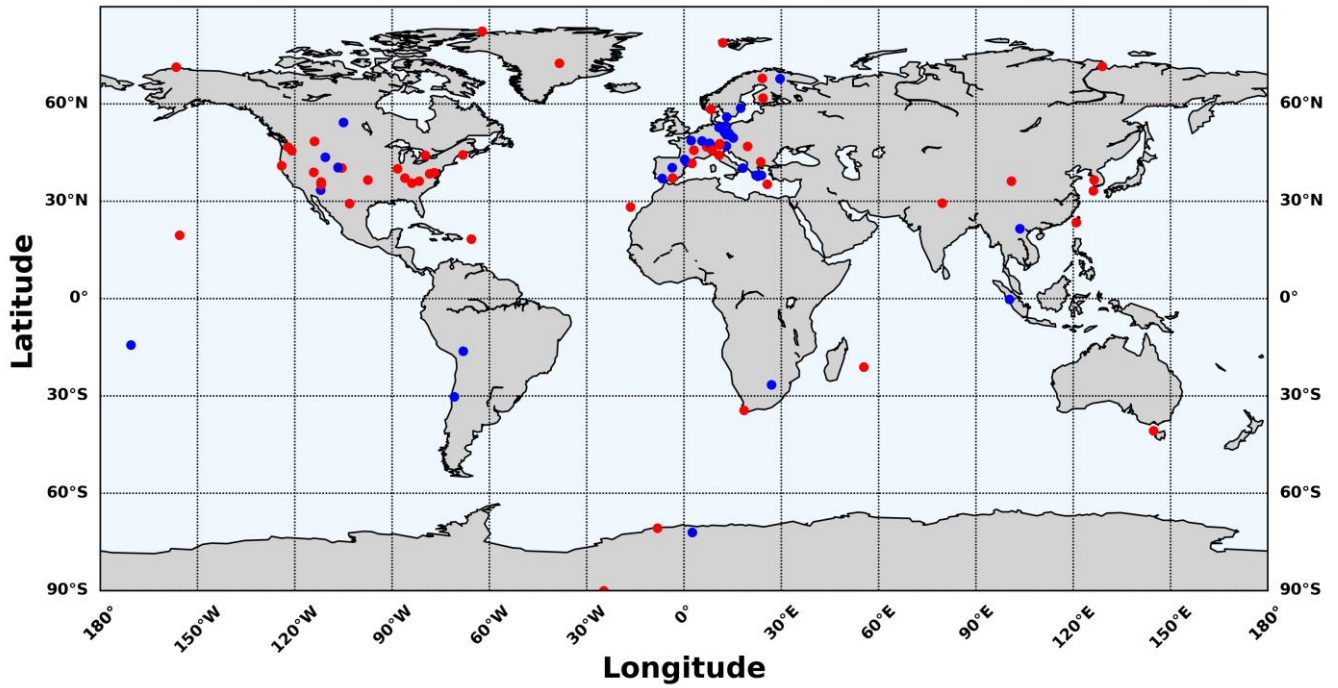
1965 Figure 1: Location of sites contributing to the present study. In blue, sites which provided information for the reference year 2017 and in red, sites that in addition, provided >10year time series for optical properties used in Collaud Coen et al. (in review, 2020).
