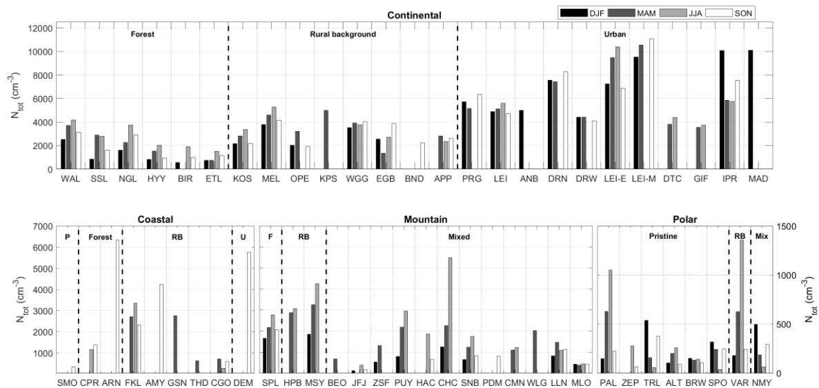
Figure 9: Seasonal medians of the total particle number concentration ( N_{tot} ). Stations are grouped according to their geographical category, and are further sorted based on their dominant footprint. For each site/season, statistics are only presented when corresponding data availability is >75\% . Note that the same scale is used for coastal and mountain sites.
