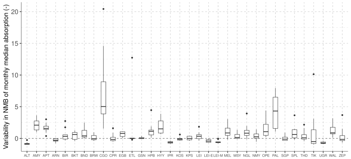
2020 Figure 10a: Boxplots of the Normalised Mean Bias (NMB) for each SARGAN site, based on monthly median in-situ observation and the corresponding monthly median AeroCom simulation result. For scattering coefficient.
