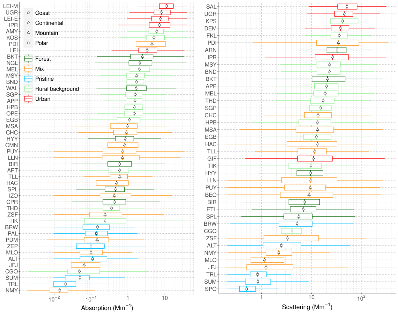
Figure 5. Boxplot of hourly aerosol absorption (left panel) and scattering (right panel) coefficients at the SARGAN sites with sufficient annual coverage over the considered period (see summary Tables SM1 and SM2 for details). Boxplot colour indicates the footprint, the symbol at the median indicates the geographical category; both colour and symbol follow Table 3.
