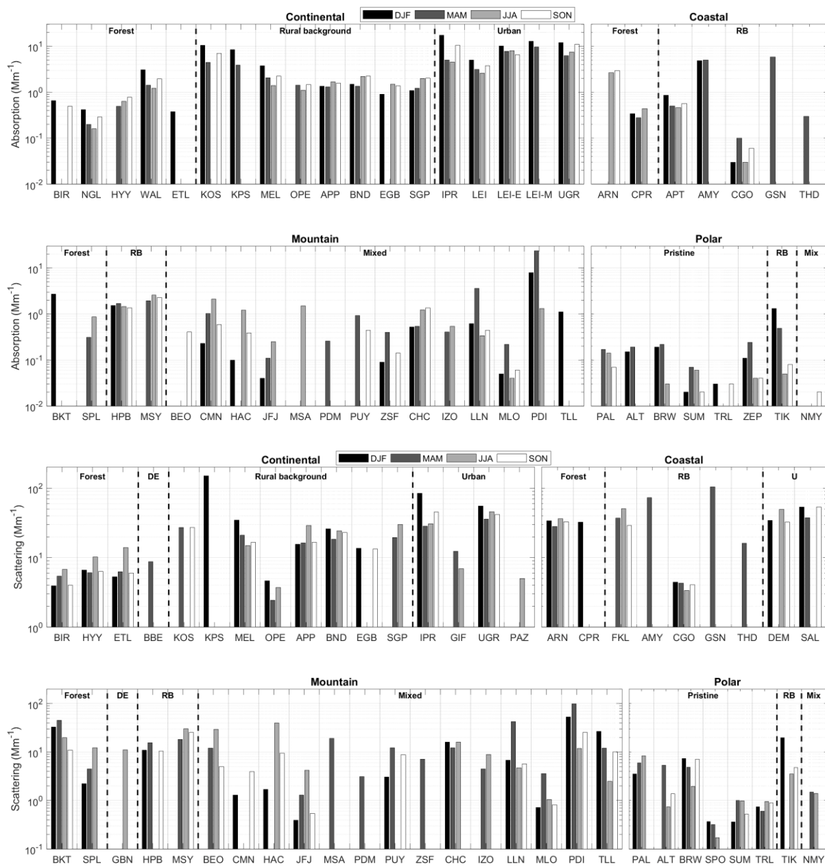
Figure 6: variation of the seasonal median of absorption coefficient (upper panel) and scattering coefficient (lower panel) for the different sites, grouped according to site classification of Table 3 with DE (Desert), U (Urban) and RB (Rural Background)
