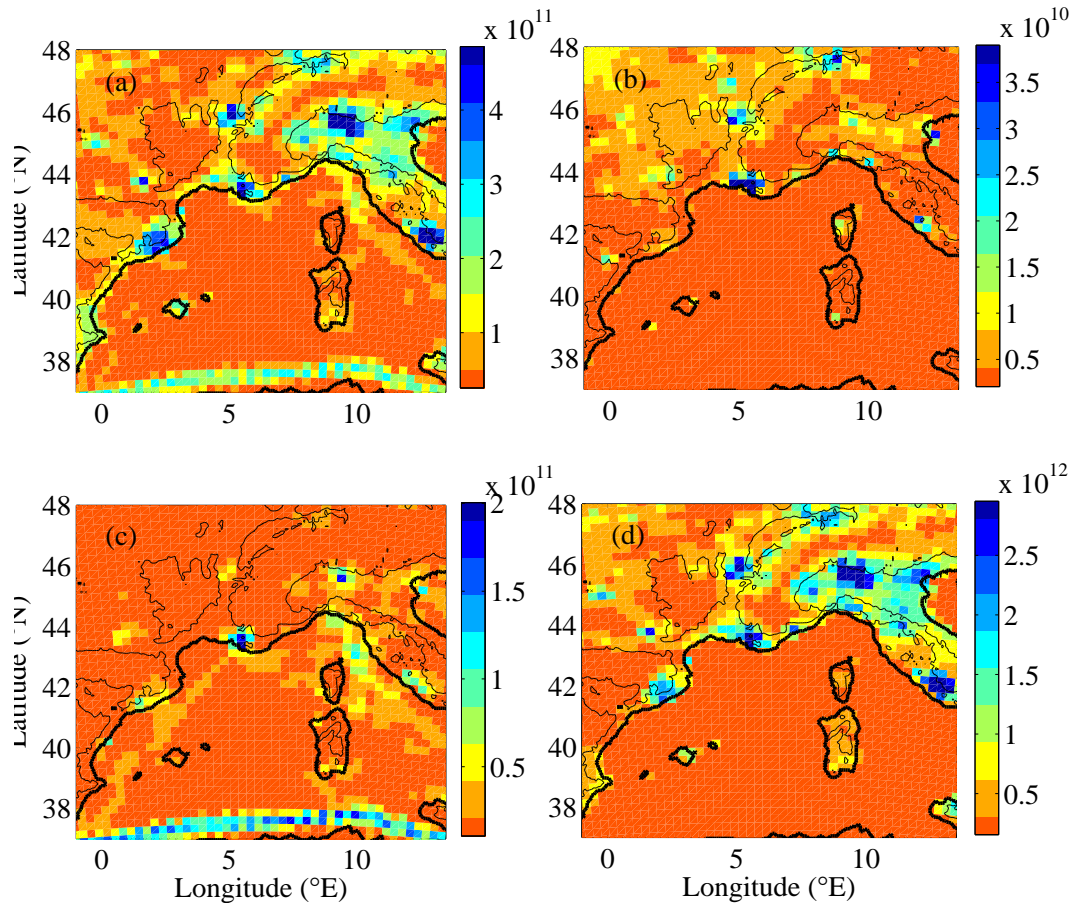
Fig. 7. EMEP inventory emissions in \text{Mg}/(50 \text{ km} \times 50 \text{ km})/\text{year} , adjusted on the grid of the domain 3 at 12:00 UTC. Panels (a), (b), (c) and (d) represent the concentrations of NO (a), PPM coarse particles ( \geq 2.5 \mu\text{m} and \leq 10 \mu\text{m} ) (b), \text{SO}_2 (c) and CO (d) during a labor day of March 1998.
