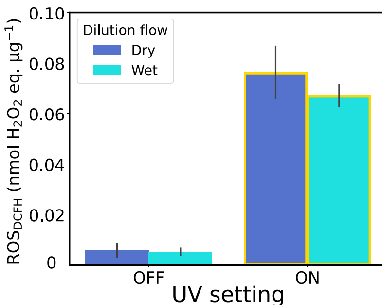
Figure A1. ROS concentrations ( \text{ROS}_{\text{DCFH}} ) from \text{Fe}^{\text{III}}\text{Cit}/\text{Cu}^{\text{II}}\text{HCit}/\text{CA} experiments in air at different humidities (RH) and dilution flow conditions (dry = blue, wet = cyan). The gray bar denotes the standard deviation of the experiments at same conditions.
