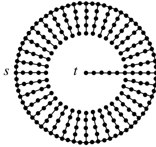
Figure 11: Lower bound construction for geographic routing algorithms [50]
