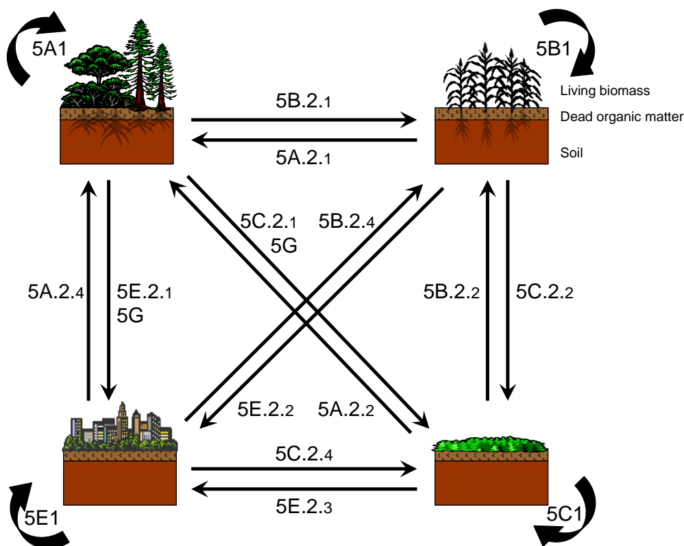
Figure 1: UK Sector 5 land use transitions showing categories for carbon stock change. See text for details.
