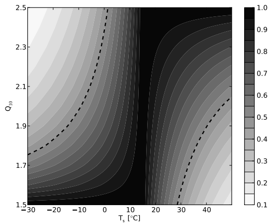
Figure 5. Values of f_T as a function of T_s and Q_{10} . For each temperature, the value is expressed as the proportion of the maximum value achieved for any value of Q_{10} . Areas outside of the dashed lines represent where f_T is less than 50 % of the maximum for the same temperature.
