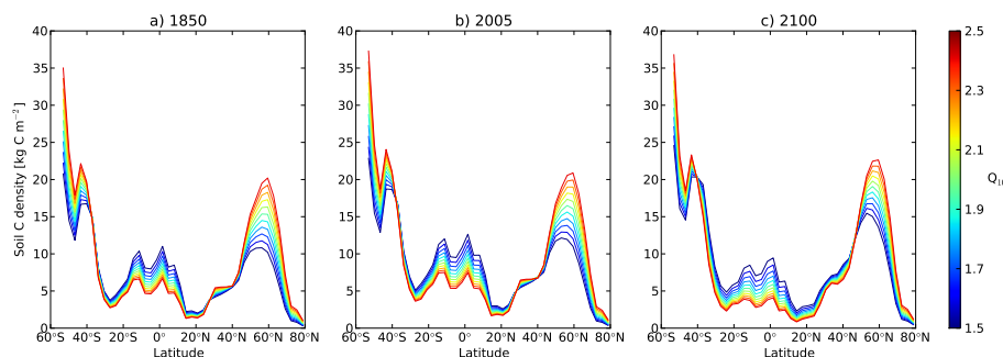
Figure 6. Zonal average soil carbon density in the reduced complexity model with k = 180 months and various values of Q_{10} as indicated by the colour bar.
