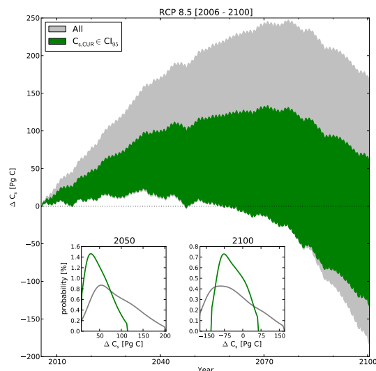
Figure 4. Change in total soil carbon through time for RCP 8.5 projections. Insets represent the probability density function of the change since 2005 for the indicated year. Grey is for all simulations while green is used to distinguish simulations for which total soil carbon is within the CI_{95} of the Harmonized World Soil Database in 2005.
