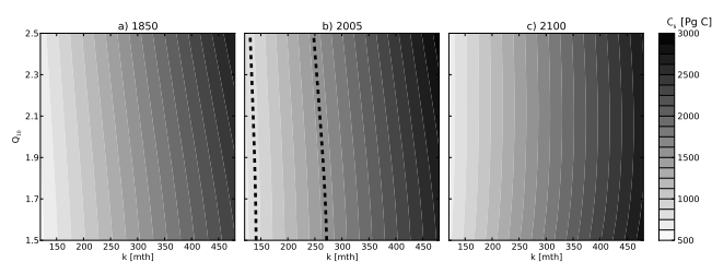
Figure 1. Snapshots of total soil carbon in the reduced complexity model as a function of parameter values. Dashed contours in panel (b) indicate the CI_{95} of the Harmonized World Soil Database in 2005 (830–1550 Pg C).
