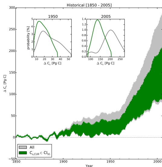
Figure 3. Change in total soil carbon through time for historical simulations. Insets represent the probability density function of the change since 1850 for the period indicated. Grey is for all simulations while green is used to distinguish simulations for which total soil carbon is within the CI_{95} of the Harmonized World Soil Database in 2005.
