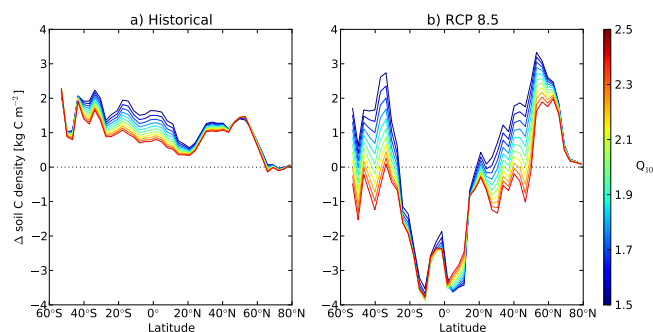
Figure 7. Zonal change in soil C density during historical simulations (a) and RCP 8.5 (b).
