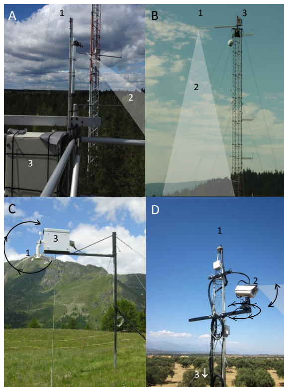
Figure 4. Hyperspectral systems in use before and during EUROSPEC. The UNIEDI System (a), the S-FLUOR/MRI System (b), the HSI System in which both the up- and down-welling measurements are hemispherical (c) and the AMSPEC-MED System where the spectrometer measuring up-welling radiance can measure at multiple zenithal and azimuthal angles (d). Down-welling hemispherical foreoptics (1), up-welling conical-FOV foreoptics (2) and the box housing the spectrometer(s) (3) are marked in the respective panels.
