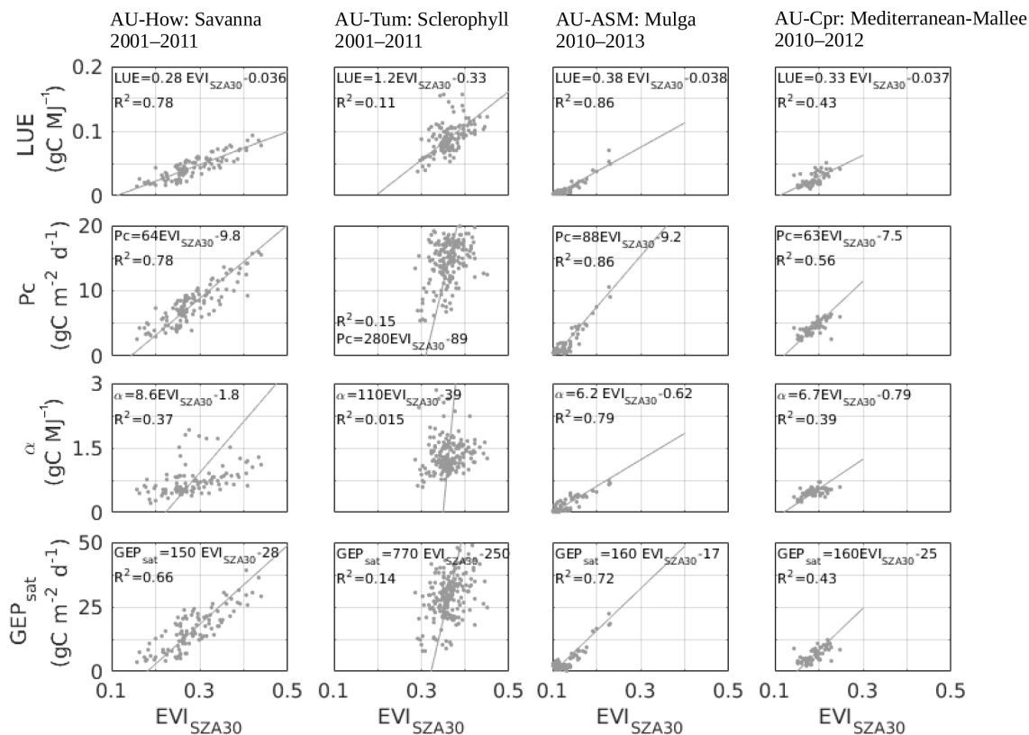
Figure 6. Relationships between 16-day mean values of (a) light use efficiency (LUE; \text{gC MJ}^{-1} ), (b) photosynthetic capacity (Pc; \text{gC m}^{-2} \text{d}^{-1} ), (c) ecosystem quantum yield ( \alpha ; \text{gC MJ}^{-1} ), and (d) GEP at saturation light ( \text{GEP}_{\text{sat}} ; \text{gC m}^{-2} \text{d}^{-1} ), and MODIS fixed solar zenith angle of 30^\circ enhanced vegetation index ( \text{EVI}_{\text{SZA30}} ). Four key Australian ecosystem sites, from left to right (columns): AU-How savanna, AU-ASM mulga, wet sclerophyll forest of AU-Tum, and AU-Cpr mallee.
