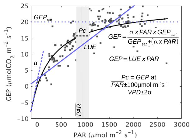
Figure 2. Rectangular hyperbola fitted to 16 days worth of hourly gross ecosystem productivity (GEP, \mu\text{molCO}_2 \text{ m}^{-2} \text{ s}^{-1} ) vs. photosynthetic active radiation (PAR, \mu\text{mol m}^{-2} \text{ s}^{-1} ) data measured at Howard Springs eddy covariance tower (black line). From the rectangular hyperbola: quantum yield ( \alpha , \mu\text{molCO}_2 \mu\text{mol}^{-1} ) (blue dashed line) and GEP at saturation ( GEP_{sat} , \mu\text{molCO}_2 \text{ m}^{-2} \text{ s}^{-1} ) (blue dotted line). Photosynthetic capacity ( Pc , \mu\text{molCO}_2 \text{ m}^{-2} \text{ s}^{-1} ) (black dashed line) was calculated as the 16-day mean GEP at mean annual daytime PAR ( PAR \pm 100 \mu\text{mol m}^{-2} \text{ s}^{-1} ) (grey area) and mean annual VPD ( VPD \pm 2 standard deviations). Light use efficiency (LUE, \mu\text{molCO}_2 \mu\text{mol}^{-1} ) was defined as the ratio between daily GEP and PAR, the slope of the linear regression (blue line).
