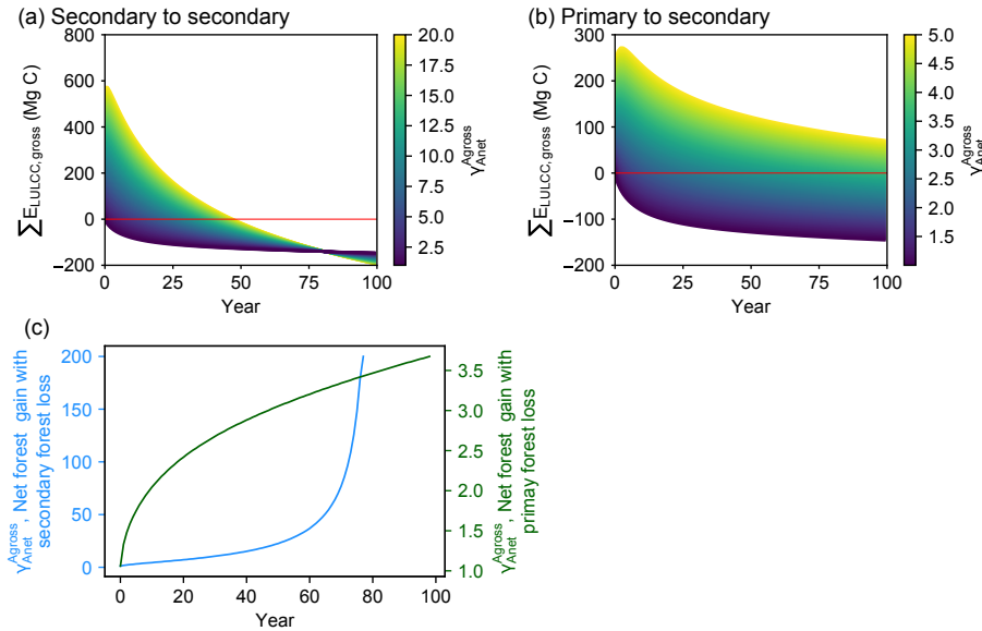
Figure 4. Time evolution of cumulative carbon flux ( \Sigma E_{LULCC, gross} ) after an initial forest area change involving gross forest area changes followed by no forest area change. The three panels show results of our bookkeeping model for three case studies. (a) A net forest gain at t = 0 with initial secondary forest loss followed by secondary forest regrowth (secondary to secondary; C1 in Table 2), (b) the same net area gain at t = 0 with initial primary forest loss followed by secondary forest regrowth (primary to secondary; C2 in Table 2) and (c) the critical value of \gamma_{A_{net}}^{A_{gross}} at which \Sigma E_{LULCC, gross} is zero, going from a net source to a net sink for a different time horizon on the x axis. The coloured curves in panels (a) and (b) have the same net area change ( A_{net} = +1 ha) at t = 0 but variable values of the initial gross-to-net area change ratios ( \gamma_{A_{net}}^{A_{gross}} ). The red line in panels (a) and (b) is the zero line, defining the time after initial forest area change at which the system reaches a neutral carbon balance. The blue and green lines in panel (c) represent the critical ratios for a net initial forest gain scenario with secondary-to-secondary (a) and primary-to-secondary (b) gross forest area change respectively. Values larger than this critical value indicate that the initial forest area change has the net effect to emit CO_2 for a given time horizon on the x axis. An exponential curve from Hansis et al. (2015) for carbon loss in all pools and gain in soil pool and a logarithmic curve from Poorter et al. (2016) for gain in biomass pool are used in this example (Table 2).
