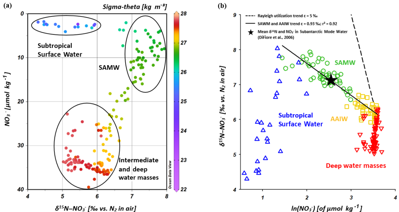
Figure 9. Nitrate concentrations vs. \delta^{15}\text{N}-\text{NO}_3^- (a) and \delta^{15}\text{N}-\text{NO}_3^- vs. \ln(\text{NO}_3^-) (b) for CTD stations within the IOSG (20.36–27.78° S). The colour code of dots in Fig. 9a indicates the potential density sigma-theta ( \text{kg m}^{-3} ). In Fig. 9b, data are grouped for the Subtropical Surface Water (blue), SAMW (green), AAIW (yellow) and deep water masses (red).
