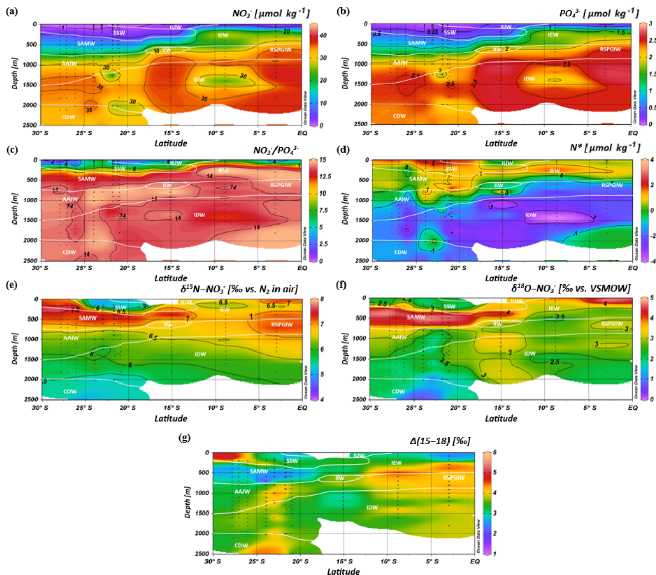
Figure 7. Latitudinal profiles from south to north with an overlay of the water mass distribution model (white contour lines) in the southern Indian Ocean for nitrate (a) and phosphate (b) concentrations, the \text{NO}_3^-/\text{PO}_4^{3-} ratio (c), \text{N}^* (d), \delta^{15}\text{N}-\text{NO}_3^- (e) and \delta^{18}\text{O}-\text{NO}_3^- of nitrate (f) and nitrate \Delta(15-18) as the difference between \delta^{15}\text{N}-\text{NO}_3^- and \delta^{18}\text{O}-\text{NO}_3^- . For water mass abbreviations see Fig. 6.
