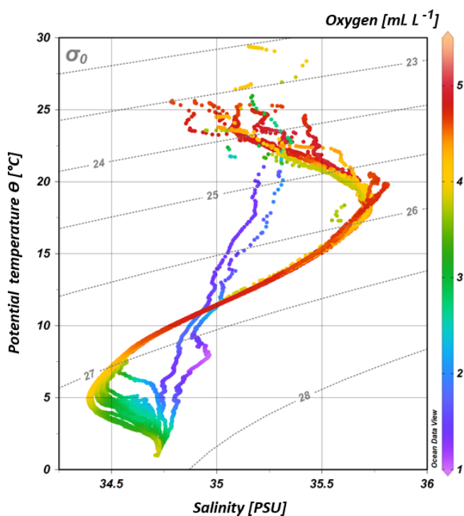
Figure 3. T–S (potential temperature vs. salinity) diagram from CTD measurements during the MSM 59/2 (2016) and SO 259 (2017) cruises. The colour bar indicates oxygen concentrations, and the grey, dotted lines represent density surfaces in sigma-theta ( \text{kg m}^{-3} ). The northernmost CTD stations (CTD 01, CTD 03; 2017) are characterized by low oxygen concentrations ( < 2 \text{ mL L}^{-1} ) and less variation in the salinity distribution, whereas the water column profiles in the IOSG indicate a distinct salinity maximum and minimum, respectively.
