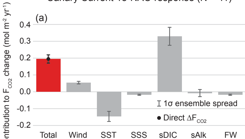
Canary Current 1 \sigma NAO response (N = 11)
