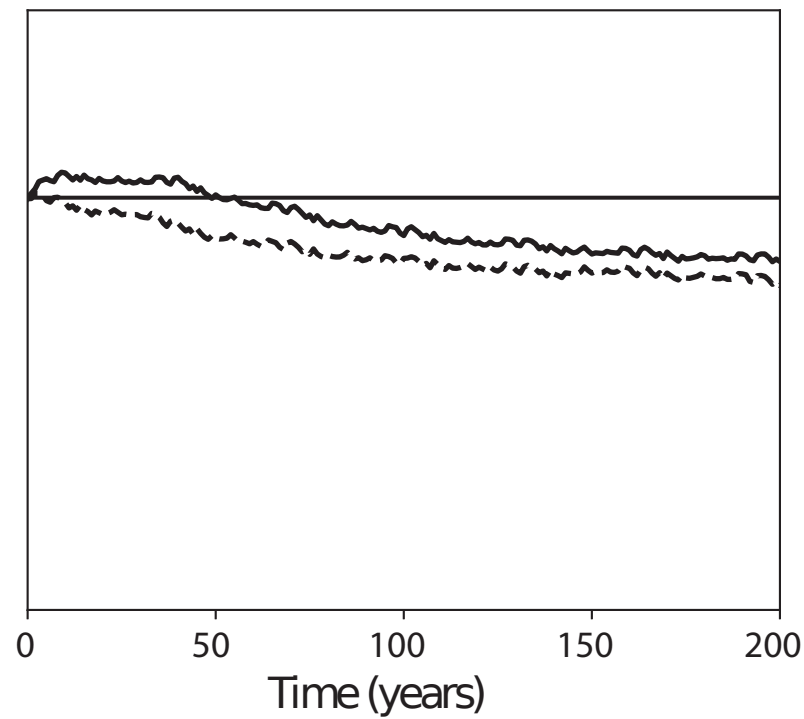
LOVECLIM 1.2
