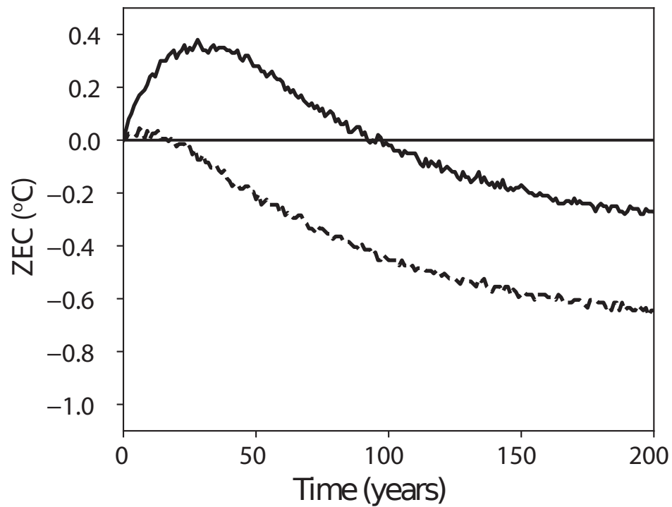
MIROC-lite
