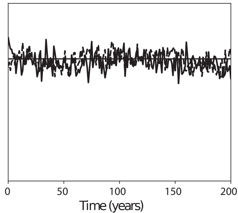
PLASIM-GENIE
