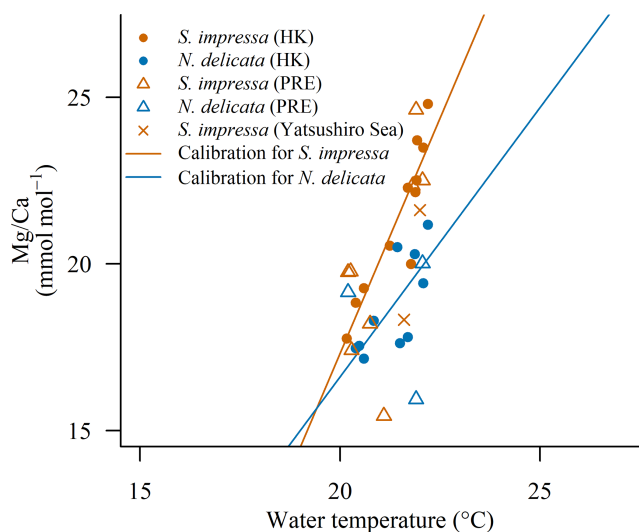
Figure 5. Mg/Ca ratios of ostracods from the PRE (OCEAN-HK) and Yatsushiro bay over the calibration for S. impressa ( \text{Mg/Ca}_{S.impressa} = 2.8 \cdot T - 39.2 ) and N. delicata ( \text{Mg/Ca}_{N.delicata} = 1.6 \cdot T - 15.7 ) performed with samples from Hong Kong (EPD). The BWT from the Copernicus product was used for OCEAN-HK samples. Surface water temperature from the Tanoura buoy in the last 15 d in June (21.8 °C) and November (21.9 °C) were considered for the Yatsushiro Sea samples.
