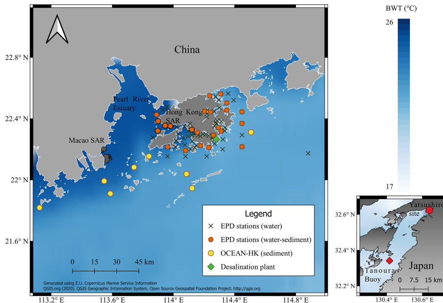
Figure 1. Sampling sites around the Pearl River estuary (PRE) and the Yatsushiro bay in Japan. Ostracods were collected from sediment samples obtained by the Environmental Protection Department of Hong Kong (EPD) and OCEAN-HK in Hong Kong. Monthly water quality data were obtained from different sampling locations across Hong Kong (EPD stations). Mean bottom-water temperature (BWT) for the year 2011 was obtained from the satellite product of the Copernicus Marine Environment Monitoring Service (CMEMS).
