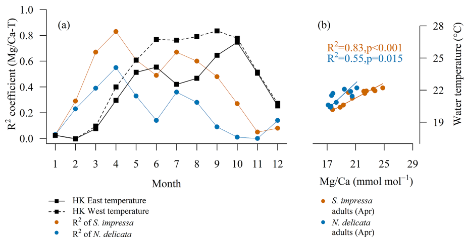
Figure 3. (a) Monthly temperature calibrations to Mg/Ca of S. impressa ( \eta = 7 ) and N. delicata ( \eta = 3 ) for adult ostracod. (b) The calibrations for S. impressa and N. delicata for April are \text{Mg/Ca}_{S. impressa} = 2.8 \cdot T - 39.2 and \text{Mg/Ca}_{N. delicata} = 1.6 \cdot T - 15.7 .
