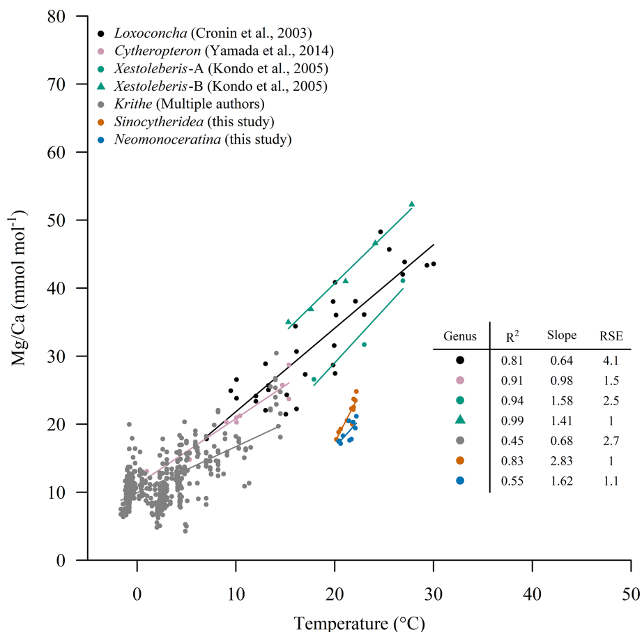
Figure 6. Temperature versus Mg/Ca ratios for specimens of the superfamily Cytheroidea . Krithe samples were retrieved from Farmer et al. (2012) and the study of Elmore et al. (2012) which contains the collection of Mg/Ca and BWT from different studies including Cadot and Kaesler (1977), Corrège and De Deckker (1997), Dwyer et al. (1995), Cronin et al. (1996), and Dwyer et al. (2002).
