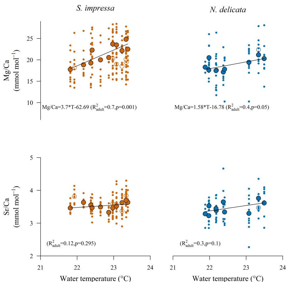
Figure 2. Relationships of Mg/Ca and Sr/Ca with annual temperature for adult (filled circles) and A-1 juvenile (open circles) ostracod samples of S. impressa ( \eta = 7 ) and N. delicata ( \eta = 3 ). Single-shell samples are shown as small dots. Solid lines show the linear regressions for adult specimens.
