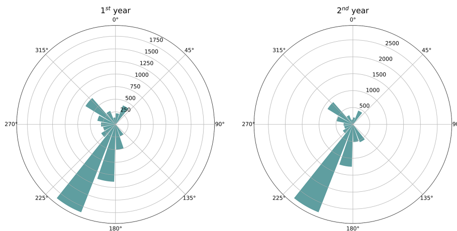
Figure 2. Number of accepted flux measurements within 20° sectors around the flux tower during the first and second years. Data from 30 to 140° were discarded.
