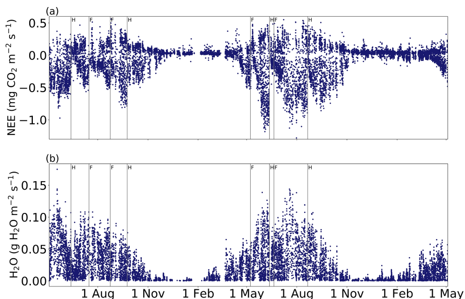
Figure 3. Accepted 30 min (a) net ecosystem exchange (NEE) and (b) H 2 O flux measurements from May 2018 to May 2020. Vertical lines with H and F indicate harvest and fertilization, respectively.
