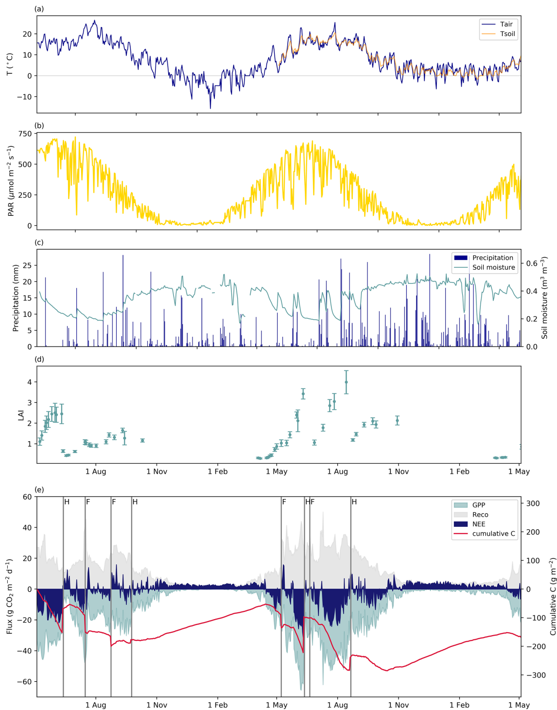
Figure 4. Daily mean (a) air and soil (depth = 0.05 m) temperature, (b) photosynthetically active radiation (PAR), (c) precipitation and soil moisture (depth = 0.1 m), (d) leaf area index (LAI), and (e) daily mean NEE, GPP, R_{\text{eco}} and cumulative carbon flux from May 2018 to May 2020.
