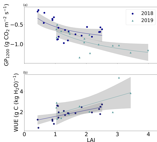
Figure 5. (a) Daily photosynthetic capacity (GP 1200 ) and (b) water use efficiency (WUE) as a function of leaf area index (LAI) during the two growing seasons. Grey areas represent the uncertainty bands.
