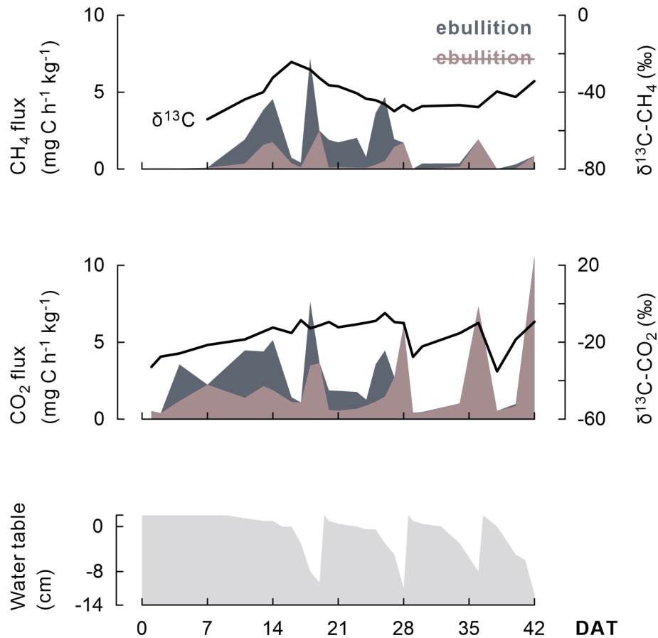
Figure 5. As this representative example (one replicate of the Balina soil with maize shoots added and under AWD) shows, the progression of CH 4 and CO 2 emission fluxes (shaded) and even their δ 13 C signature (black line) appear linked to the change in water table depth under AWD. A distinction is made between emission fluxes dominated by ebullition (dark grey shaded) versus by diffusion or plant transport (brown shaded). Transport through ebullition was particularly considerable when rice plants were juvenile.
