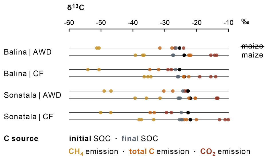
Figure 6. In the absence of maize, the overall δ 13 C signature of C emissions (values per replicate) was lower (i.e. less 13 C-enriched) under CF than under AWD ( P = 0.02 ).
