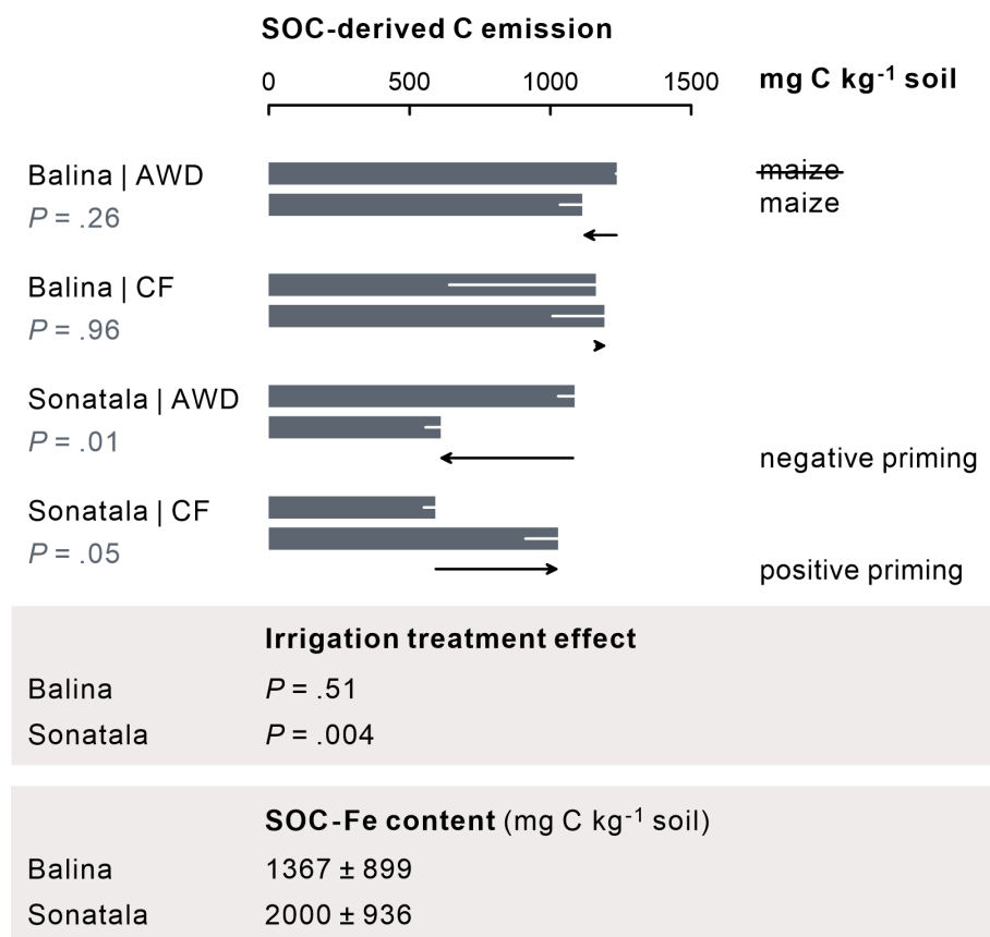
Figure 7. For the Sonatala soil, maize addition led to positive priming of gaseous C ( \text{CO}_2 + \text{CH}_4 ) emission under CF and negative priming under AWD. P -values of the priming effect significance (in the figure) and of the irrigation treatment effect on the priming effect (below the figure) are indicated. Standard errors (three or two replicates) are indicated. Fe-bound SOC levels (average \pm standard error, estimated by means of \text{NH}_2\text{OH} \cdot \text{HCl} ) exceed the positive priming effect of Sonatala under CF, so stimulated Fe-C dissolution and emission has the potential to explain this priming.
