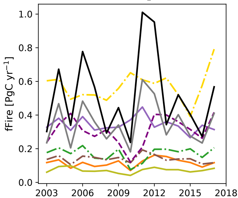
(c) Annual fire CO 2 emissions
