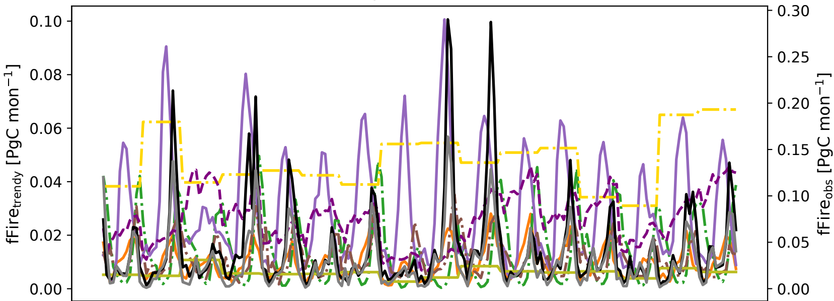
(a) Monthly fire CO 2 emissions
