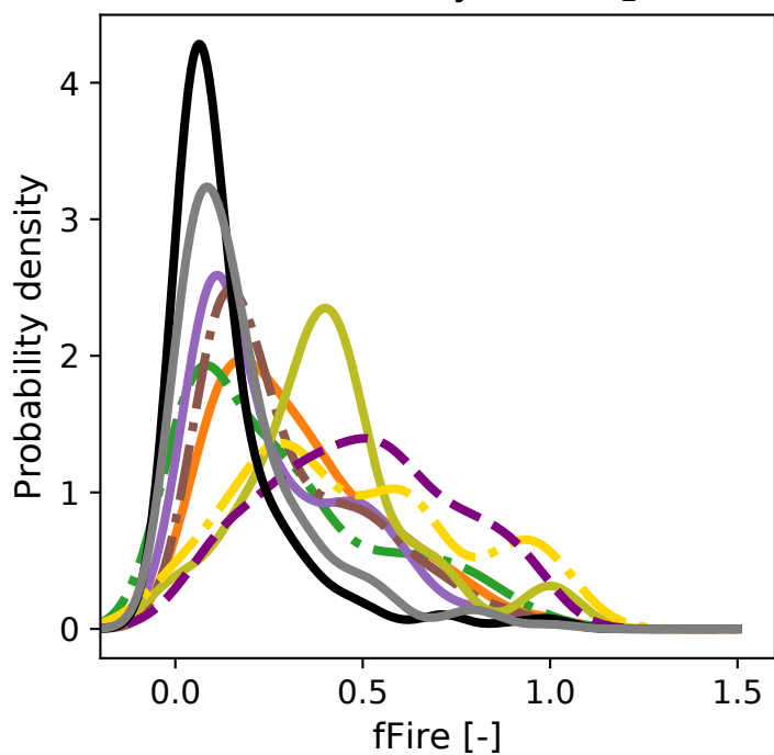
(b) Normalised monthly fire CO 2 emissions
