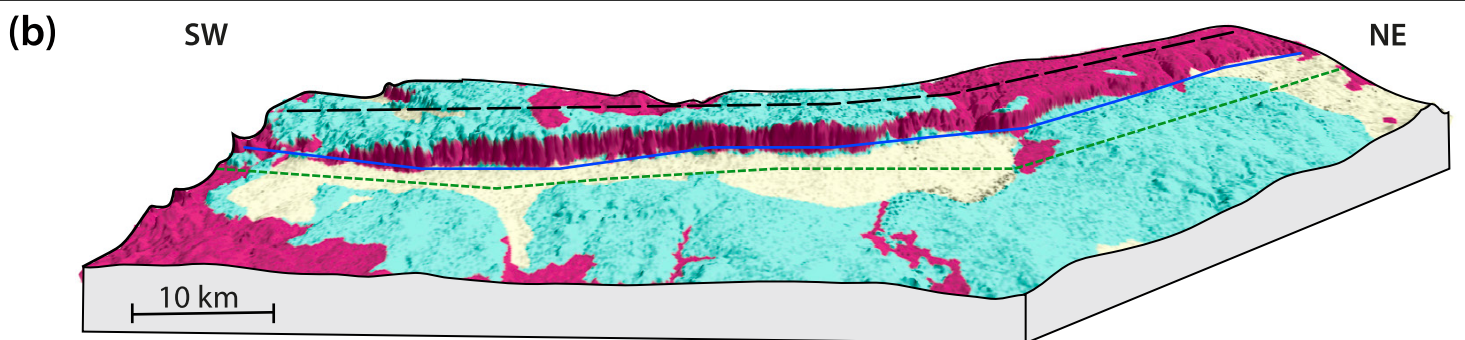
Isuria Fault
