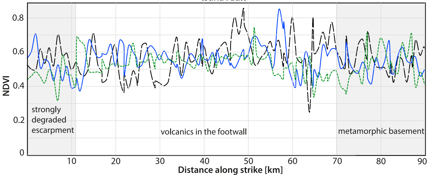
Isuria Fault
