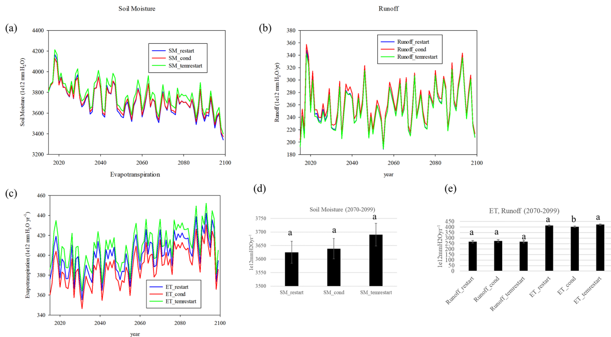
Figure 11. (a) Soil moisture, (b) runoff, and (c) evapotranspiration between the RESTART, CONDENSED, and TEMRESTART experiments; (d) mean differences 2070–2099 for soil moisture and (e) mean difference 2070–2099 for runoff and evapotranspiration (letters based on ANOVA analysis with P < 0.05 ).
