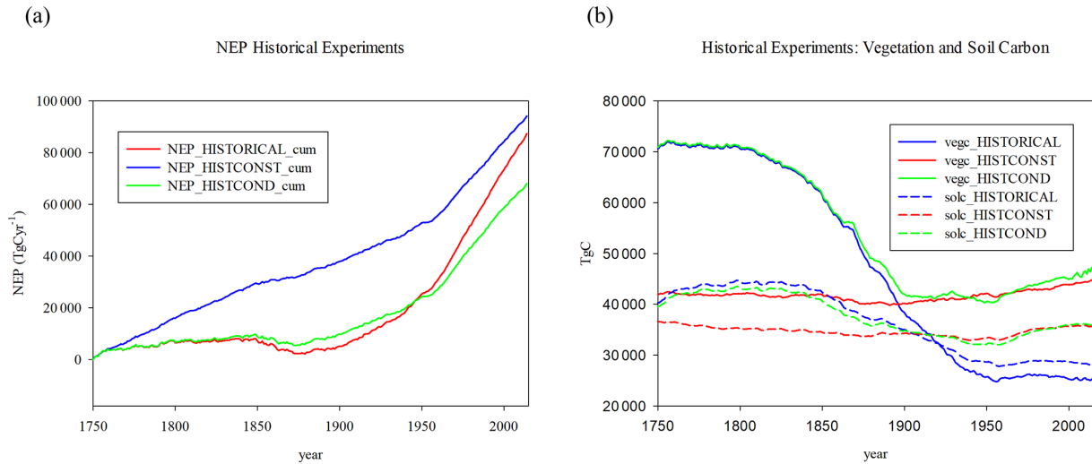
Figure 2. Historical experiments (a) cumulative NEP ( \text{TgC yr}^{-1} ), (b) vegetation carbon (vegC), and soil carbon (solC) in TgC. Experiments are HISTORICAL, HISTCONST, and HISTCOND (see text).
