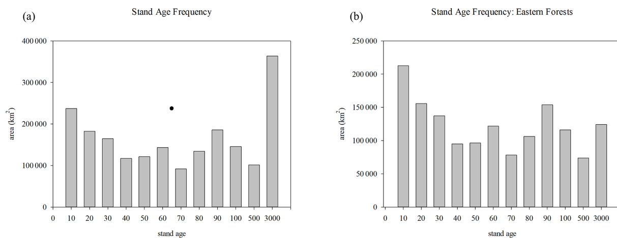
Figure 8. (a) Stand-age frequency for US and (b) eastern forests. Bins represent 0–10, 11–20, 21–30, 31–40, 41–50, 51–60, 61–70, 71–80, 81–90, 91–100, 101–500, > 500 years.
