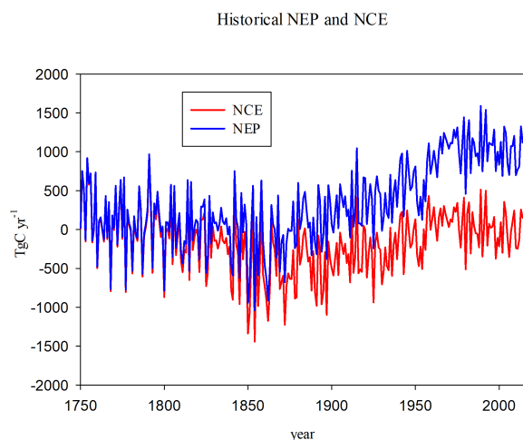
Figure 1. Net carbon exchange (NCE) and net ecosystem productivity (NEP) for the HISTORICAL run. NCE includes fluxes from agricultural conversion and abandonment and decomposition of agricultural products.
