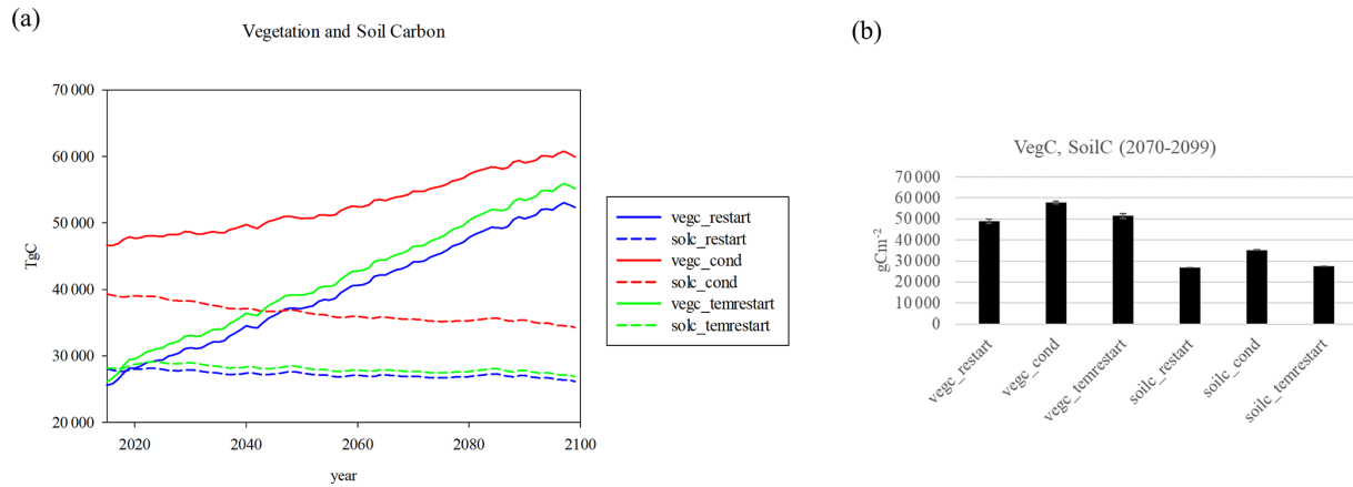
Figure 6. (a) Vegetation and soil carbon in the RESTART, CONDENSED, and TEMRESTART experiments, (b) mean differences 2070–2099 (all three vegetation carbons and soil carbons differ significantly from each other).
