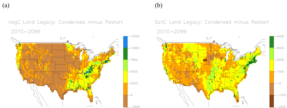
Figure 7. Mapped patterns in (a) vegetation ( -14\,350 to 13\,146\text{ gC m}^{-2} ) and (b) soil carbon ( -2489 to 9339\text{ gC m}^{-2} ) as differences between the CONDENSED and RESTART experiments.
