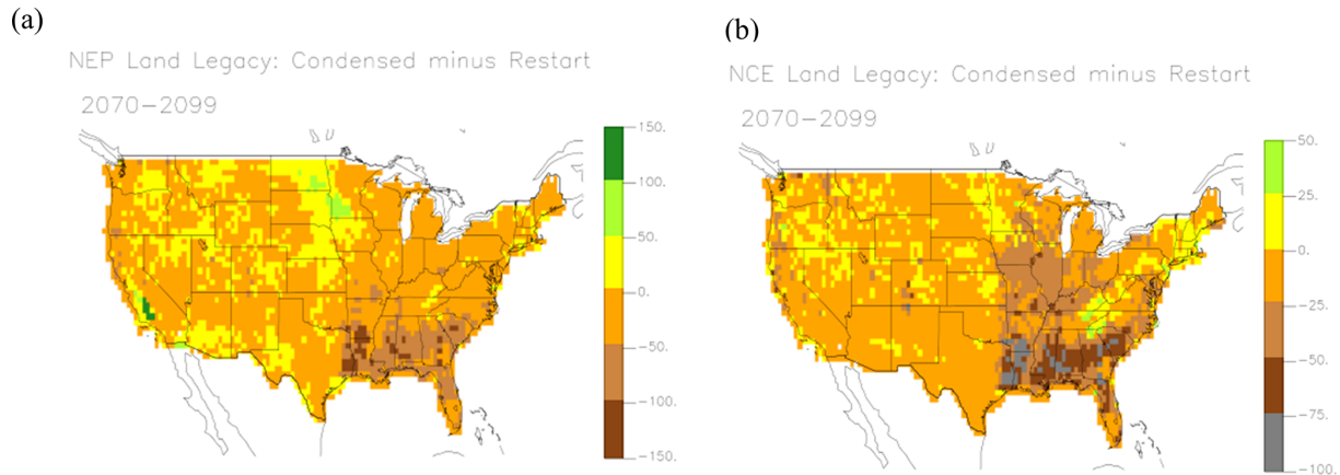
Figure 4. Mapped differences in NEP and NCE, illustrating effect of land legacy as difference between the CONDENSED and RESTART runs, (a) NEP ( -164 to 198 \text{ gC m}^{-2} \text{ yr}^{-1} ), (b) NCE ( -164 to 55 \text{ gC m}^{-2} \text{ yr}^{-1} ).
