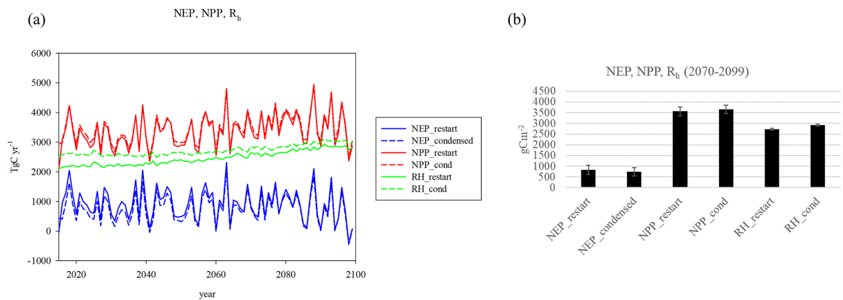
Figure 5. (a) Carbon fluxes (NEP, NPP, R_h ) for the RESTART and CONDENSED runs, (b) mean differences 2070–2099 (no significant differences for either of the three pairs).
