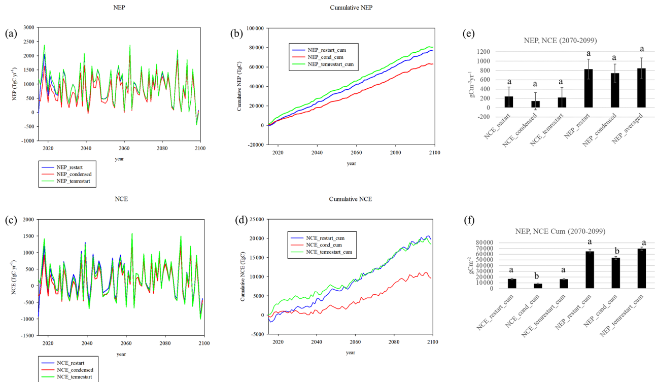
Figure 3. Comparison of NEP and NEC between the RESTART, CONDENSED, and TEMRESTART runs; (a) NEP, (b) cumulative NEP, (c) NCE, and (d) cumulative NCE; (e) NEP, NCE comparison 2070–2099 means (error bars 1 standard deviation), (f) cumulative NEP, NCE comparison, 2070–2099 means (error bars 95 % confidence interval). ANOVA analysis for (d) and (e) based on P < 0.05 .
