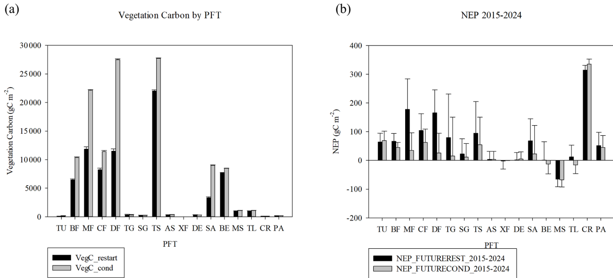
Figure 10. (a) Vegetation carbon by plant functional type in 2015 for the RESTART and for the CONDENSED experiments, (b) NEP by PFT averaged 2015–2024. PFTs are as follows: T is tundra, BF is boreal forest, MF is mixed temperate forest, CF is temperate coniferous forest, DF is temperate deciduous forest, TG is tall grasslands, SG is short grasslands, TS is tropical savanna, AS is arid shrublands, XF is xeric forests and woodlands, DE is deserts, SA is temperate savannas, BE is temperate broadleaved evergreen forests, MS is Mediterranean shrublands, TL is turf lawn, PA is pasture, and CR is crops. Error bars are 10-year interannual variability, computed as 95 % confidence interval of year 2015–2024 for each PFT in each of the two runs.
